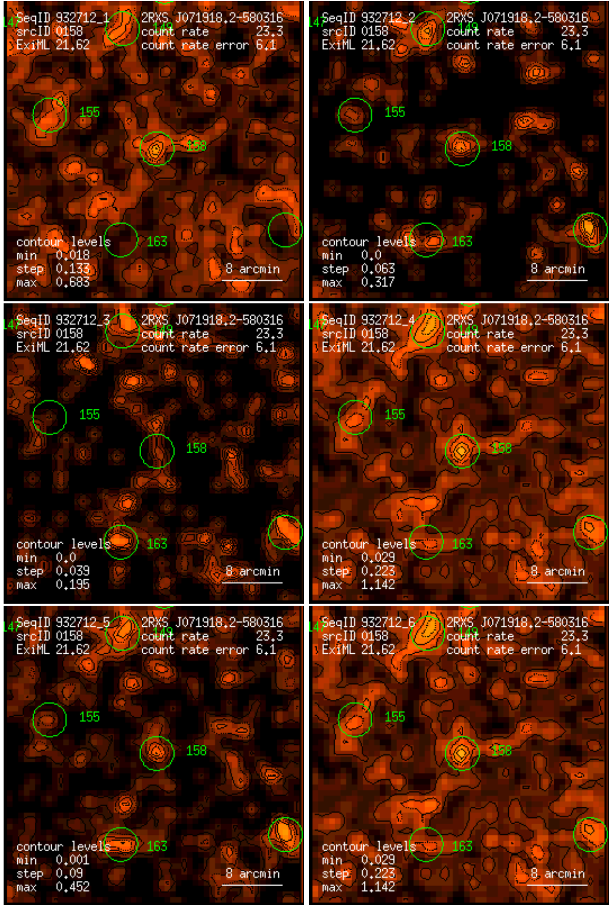
Figure 158: RASS 932712: detection 0158: band rate images, Gaussian filter: (1) PSPC channels 11 – 41, (2) 52 – 90, (3) 91 – 201, (4) 11 – 235, (5) 52 – 201, (6) 11 – 201. Broad band rates in counts/ks. Band rate contour levels in counts/ks/arcmin 2 .
