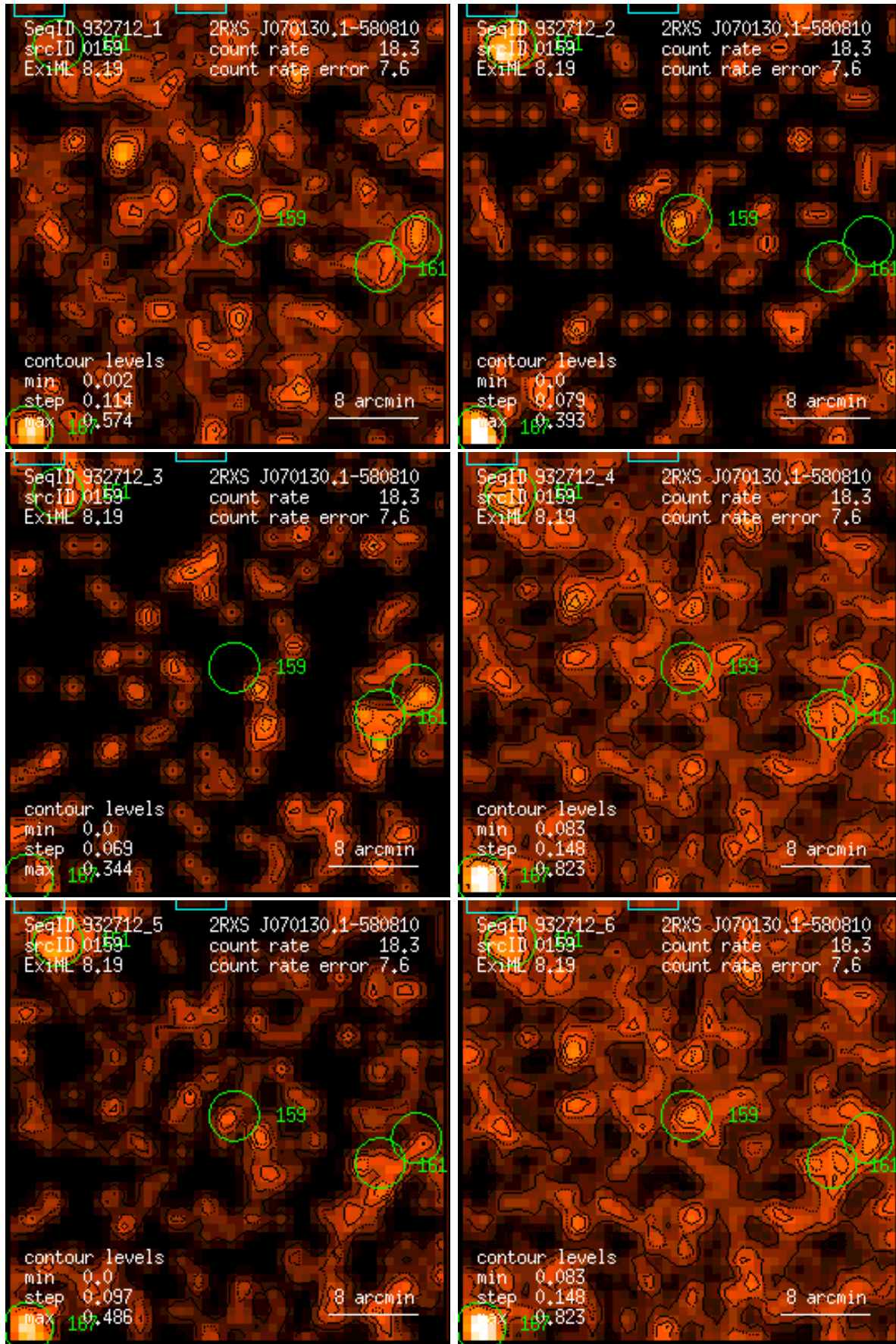
Figure 159: RASS 932712: detection 0159: band rate images, Gaussian filter: (1) PSPC channels 11 – 41, (2) 52 – 90, (3) 91 – 201, (4) 11 – 235, (5) 52 – 201, (6) 11 – 201. Broad band rates in counts/ks. Band rate contour levels in counts/ks/arcmin 2 .
