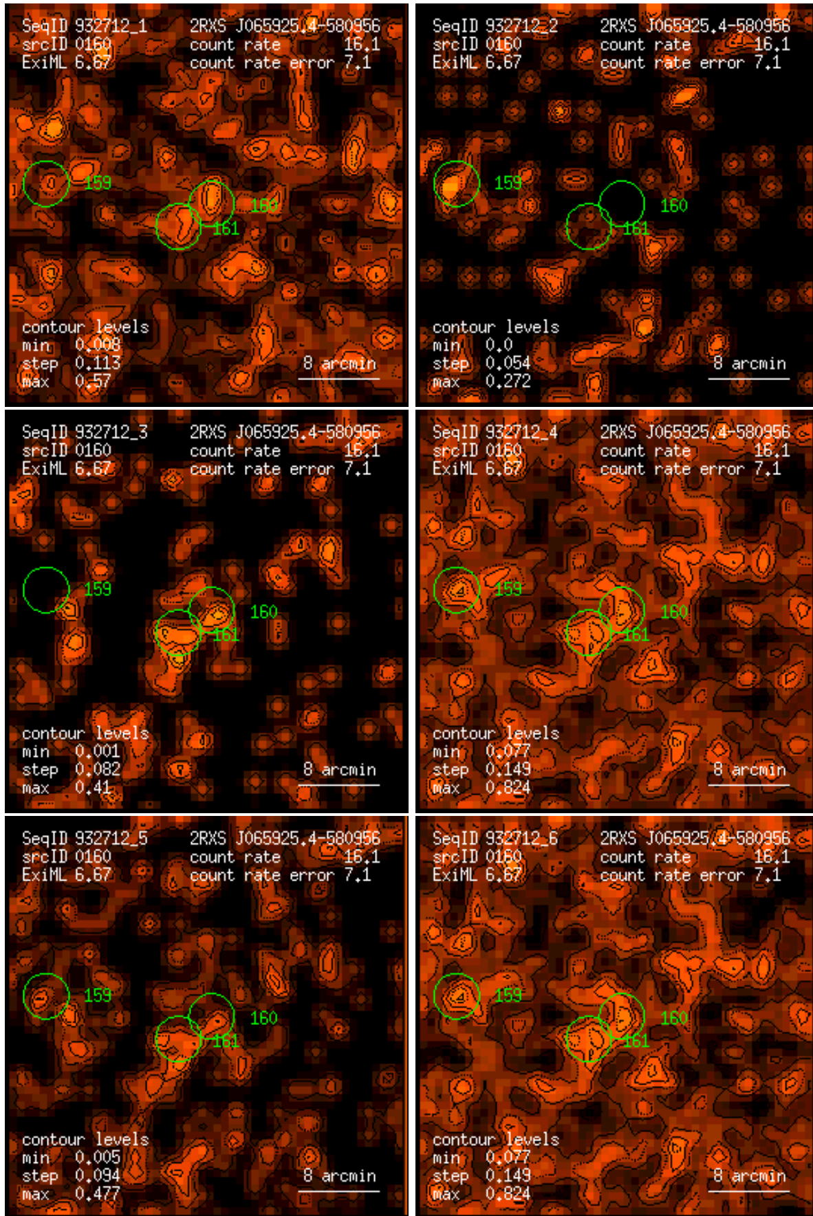
Figure 160: RASS 932712: detection 0160: band rate images, Gaussian filter: (1) PSPC channels 11 – 41, (2) 52 – 90, (3) 91 – 201, (4) 11 – 235, (5) 52 – 201, (6) 11 – 201. Broad band rates in counts/ks. Band rate contour levels in counts/ks/arcmin 2 .
