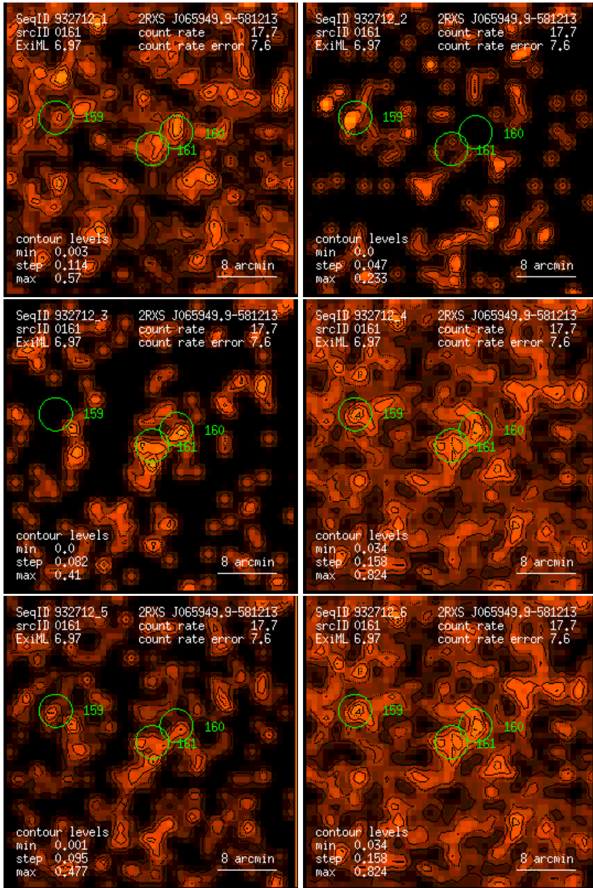
Figure 161: RASS 932712: detection 0161: band rate images, Gaussian filter: (1) PSPC channels 11 – 41, (2) 52 – 90, (3) 91 – 201, (4) 11 – 235, (5) 52 – 201, (6) 11 – 201. Broad band rates in counts/ks. Band rate contour levels in counts/ks/arcmin 2 .
