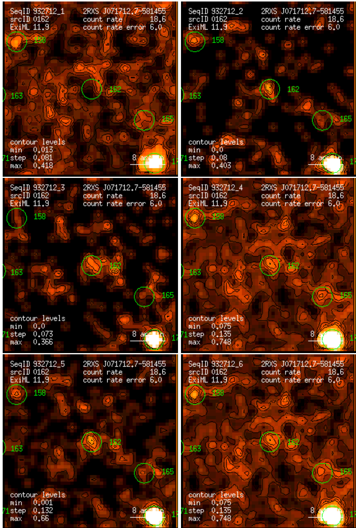
Figure 162: RASS 932712: detection 0162: band rate images, Gaussian filter: (1) PSPC channels 11 – 41, (2) 52 – 90, (3) 91 – 201, (4) 11 – 235, (5) 52 – 201, (6) 11 – 201. Broad band rates in counts/ks. Band rate contour levels in counts/ks/arcmin 2 .
