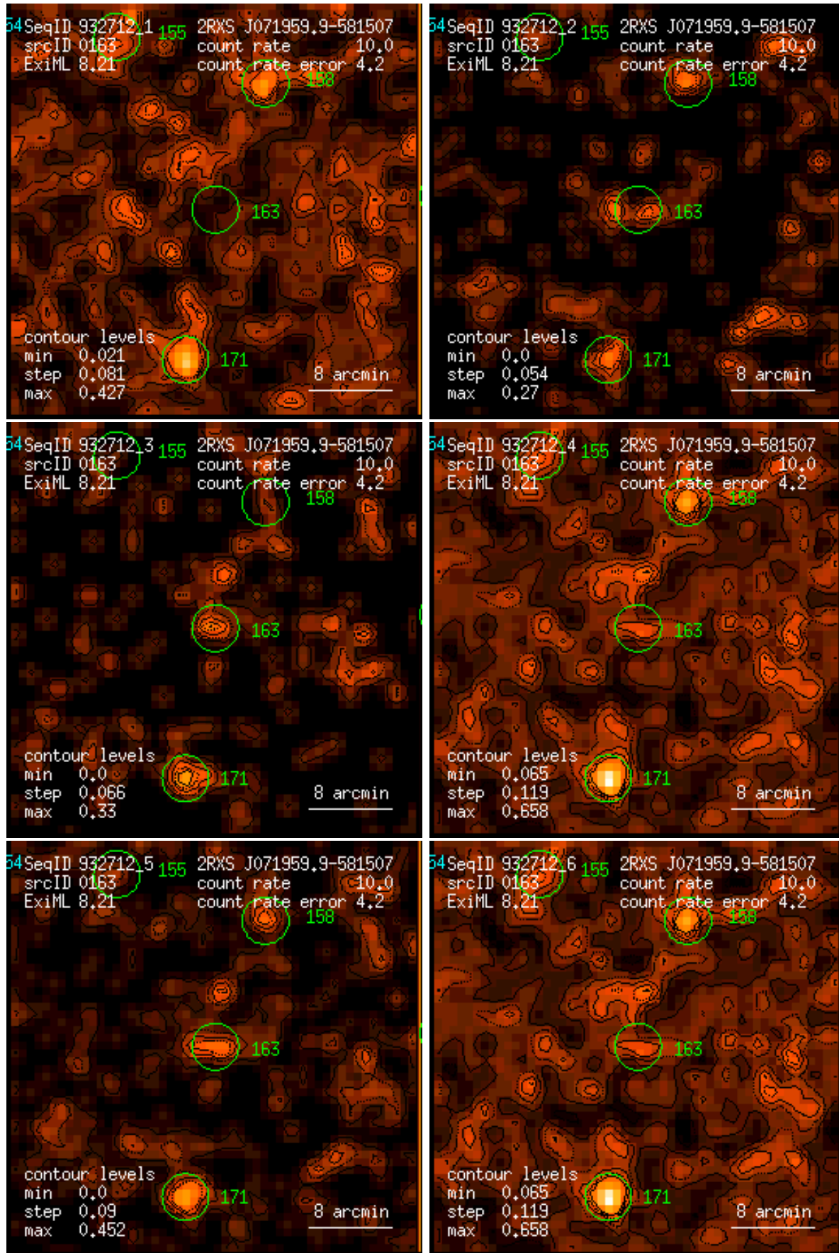
Figure 163: RASS 932712: detection 0163: band rate images, Gaussian filter: (1) PSPC channels 11 – 41, (2) 52 – 90, (3) 91 – 201, (4) 11 – 235, (5) 52 – 201, (6) 11 – 201. Broad band rates in counts/ks. Band rate contour levels in counts/ks/arcmin 2 .
