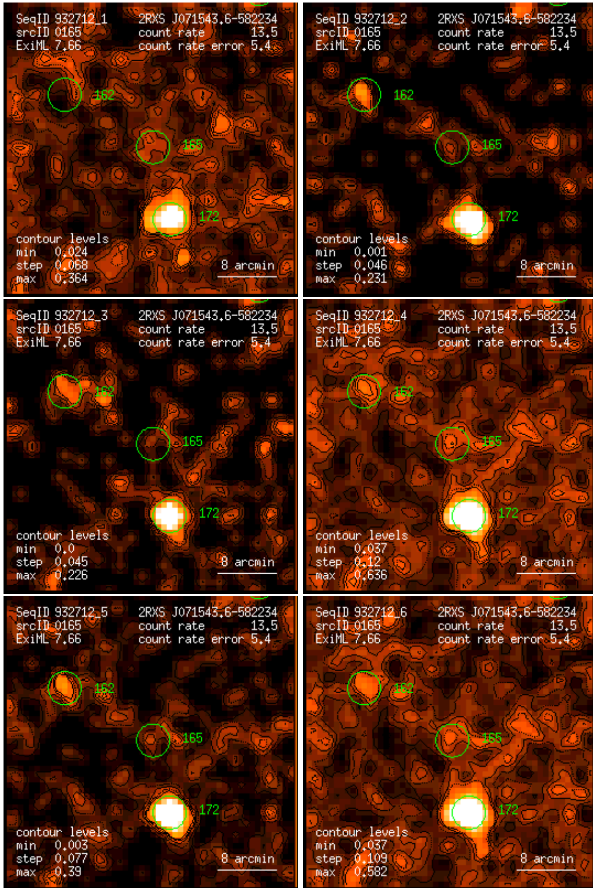
Figure 165: RASS 932712: detection 0165: band rate images, Gaussian filter: (1) PSPC channels 11 – 41, (2) 52 – 90, (3) 91 – 201, (4) 11 – 235, (5) 52 – 201, (6) 11 – 201. Broad band rates in counts/ks. Band rate contour levels in counts/ks/arcmin 2 .
