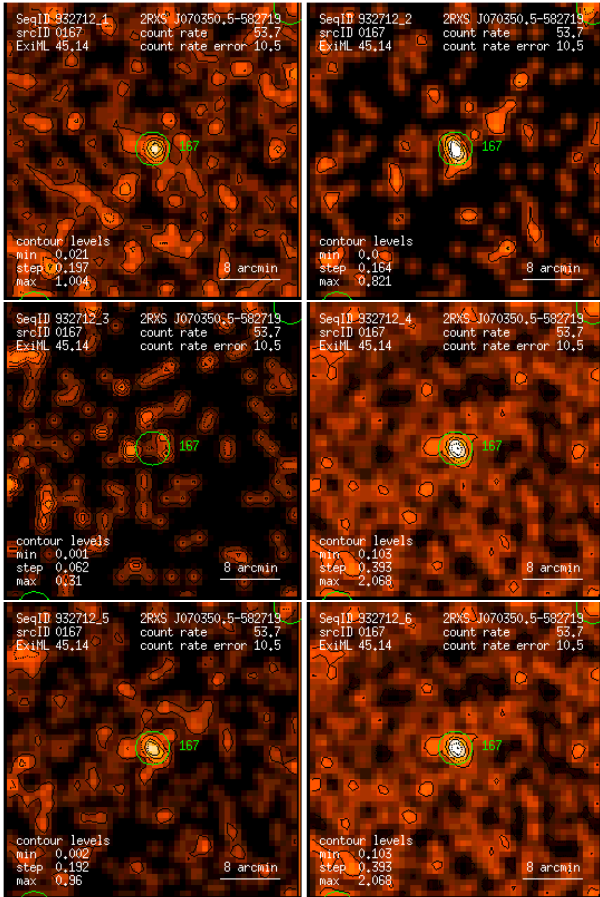
Figure 167: RASS 932712: detection 0167: band rate images, Gaussian filter: (1) PSPC channels 11 – 41, (2) 52 – 90, (3) 91 – 201, (4) 11 – 235, (5) 52 – 201, (6) 11 – 201. Broad band rates in counts/ks. Band rate contour levels in counts/ks/arcmin 2 .
