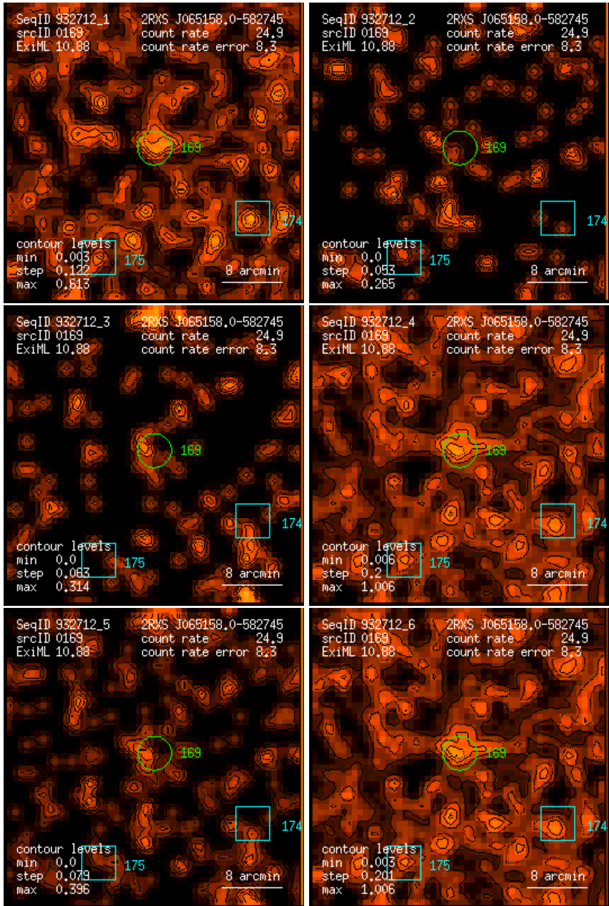
Figure 169: RASS 932712: detection 0169: band rate images, Gaussian filter: (1) PSPC channels 11 – 41, (2) 52 – 90, (3) 91 – 201, (4) 11 – 235, (5) 52 – 201, (6) 11 – 201. Broad band rates in counts/ks. Band rate contour levels in counts/ks/arcmin 2 .
