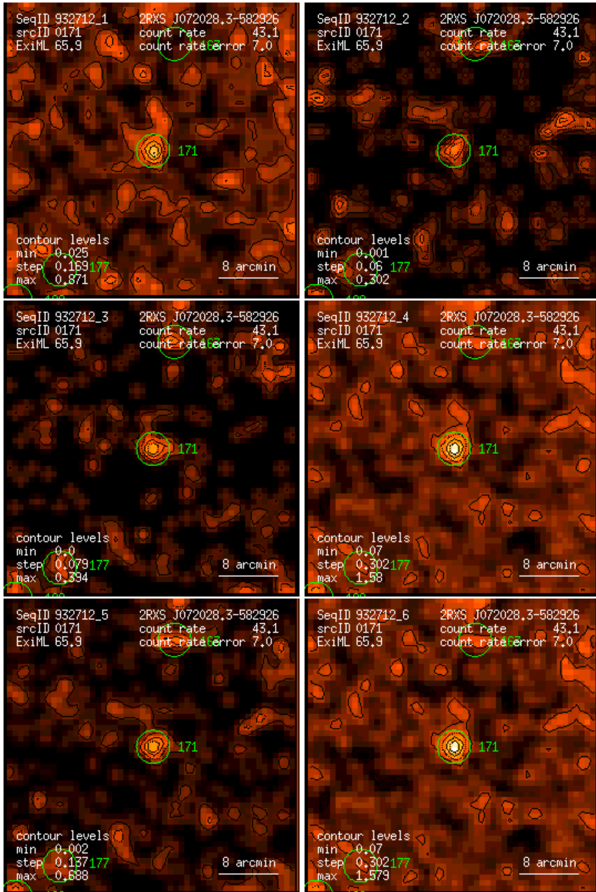
Figure 171: RASS 932712: detection 0171: band rate images, Gaussian filter: (1) PSPC channels 11 – 41, (2) 52 – 90, (3) 91 – 201, (4) 11 – 235, (5) 52 – 201, (6) 11 – 201. Broad band rates in counts/ks. Band rate contour levels in counts/ks/arcmin 2 .
