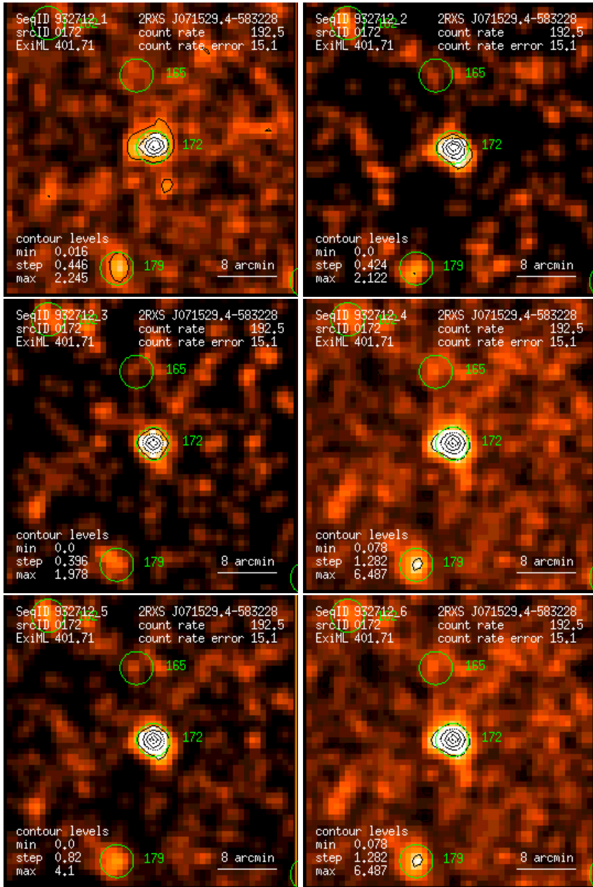
Figure 172: RASS 932712: detection 0172: band rate images, Gaussian filter: (1) PSPC channels 11 – 41, (2) 52 – 90, (3) 91 – 201, (4) 11 – 235, (5) 52 – 201, (6) 11 – 201. Broad band rates in counts/ks. Band rate contour levels in counts/ks/arcmin 2 .
