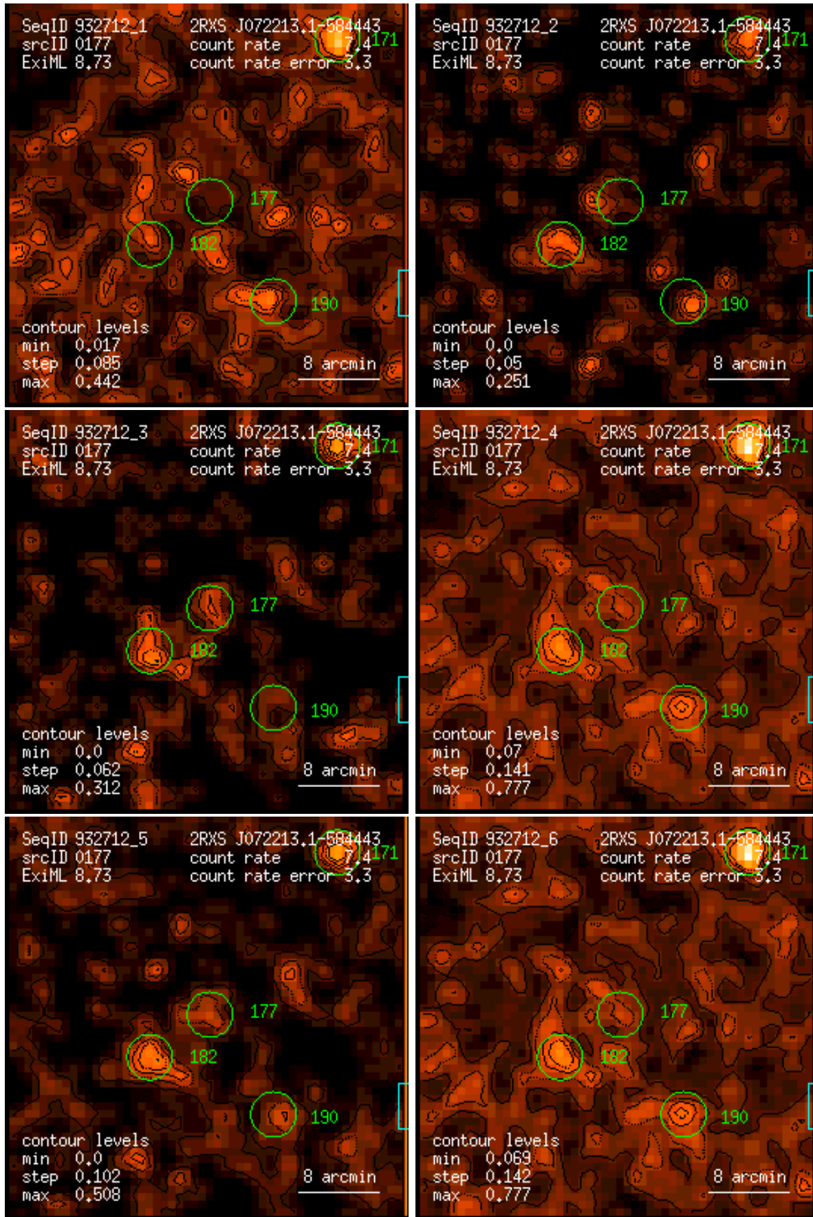
Figure 177: RASS 932712: detection 0177: band rate images, Gaussian filter: (1) PSPC channels 11 – 41, (2) 52 – 90, (3) 91 – 201, (4) 11 – 235, (5) 52 – 201, (6) 11 – 201. Broad band rates in counts/ks. Band rate contour levels in counts/ks/arcmin 2 .
