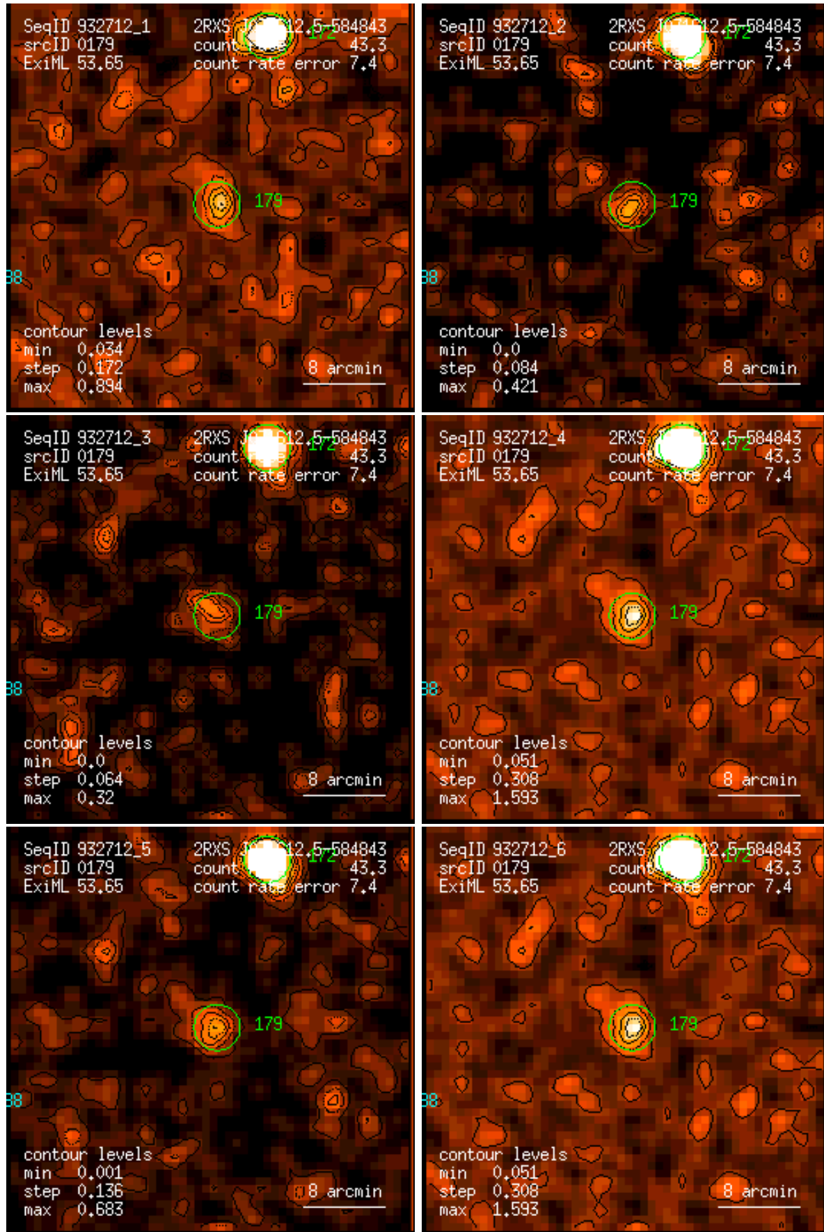
Figure 179: RASS 932712: detection 0179: band rate images, Gaussian filter: (1) PSPC channels 11 – 41, (2) 52 – 90, (3) 91 – 201, (4) 11 – 235, (5) 52 – 201, (6) 11 – 201. Broad band rates in counts/ks. Band rate contour levels in counts/ks/arcmin 2 .
