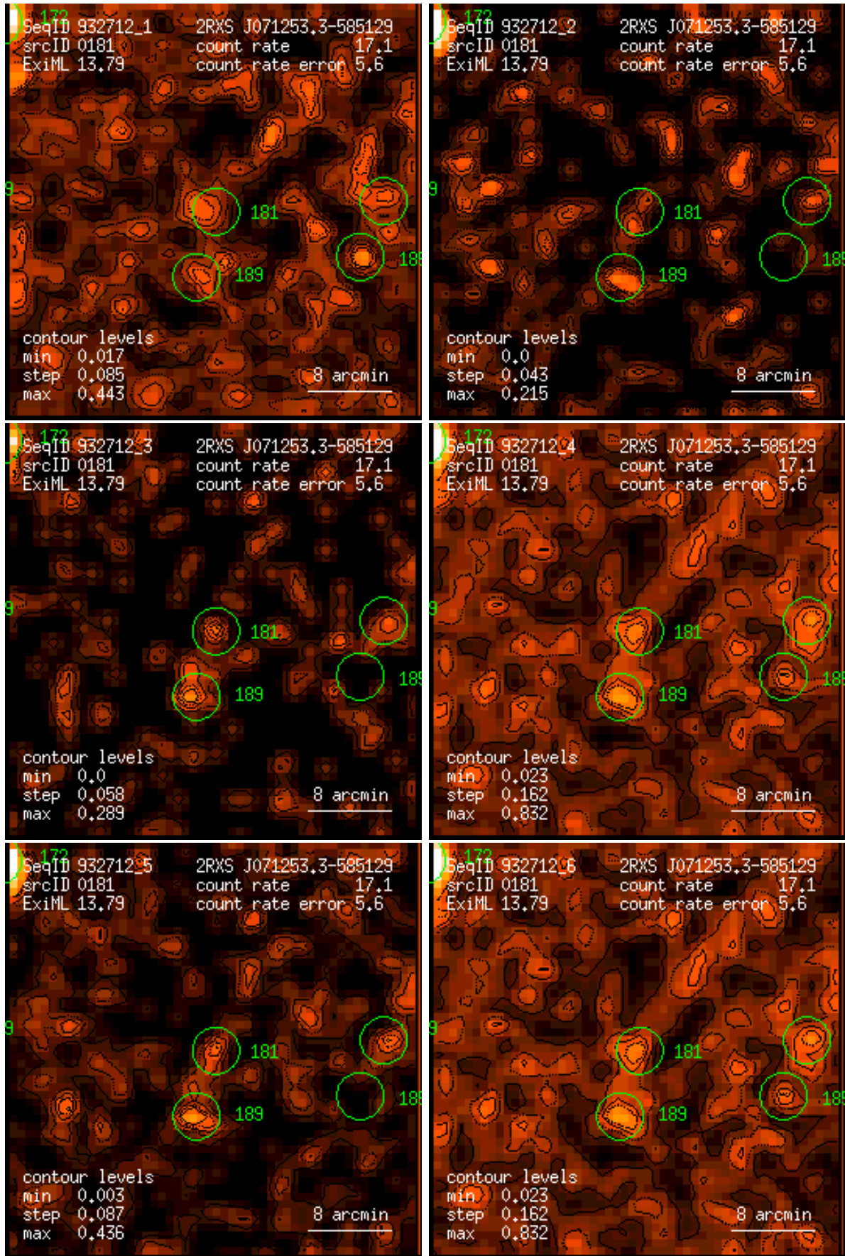
Figure 181: RASS 932712: detection 0181: band rate images, Gaussian filter: (1) PSPC channels 11 – 41, (2) 52 – 90, (3) 91 – 201, (4) 11 – 235, (5) 52 – 201, (6) 11 – 201. Broad band rates in counts/ks. Band rate contour levels in counts/ks/arcmin 2 .
