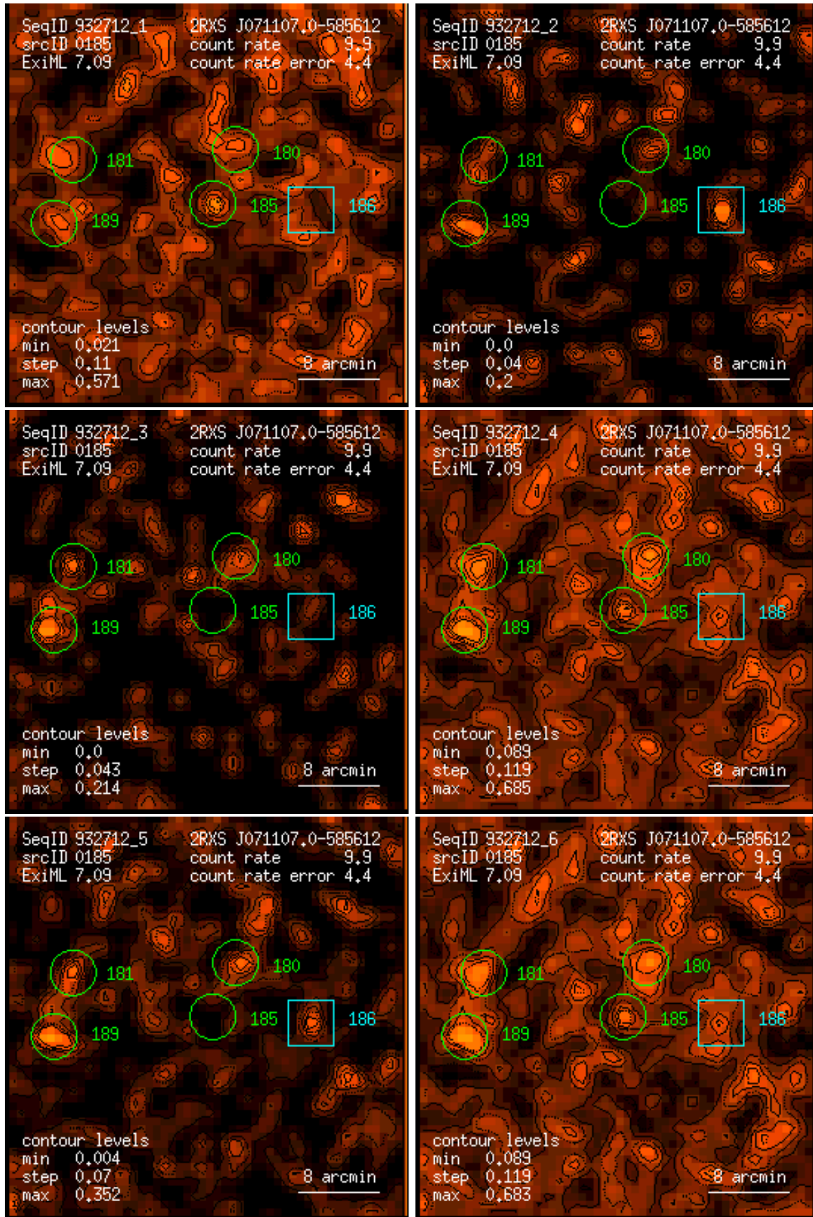
Figure 185: RASS 932712: detection 0185: band rate images, Gaussian filter: (1) PSPC channels 11 – 41, (2) 52 – 90, (3) 91 – 201, (4) 11 – 235, (5) 52 – 201, (6) 11 – 201. Broad band rates in counts/ks. Band rate contour levels in counts/ks/arcmin 2 .
