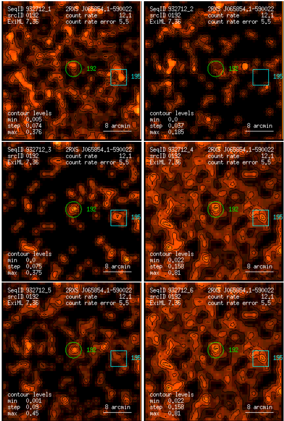
Figure 192: RASS 932712: detection 0192: band rate images, Gaussian filter: (1) PSPC channels 11 – 41, (2) 52 – 90, (3) 91 – 201, (4) 11 – 235, (5) 52 – 201, (6) 11 – 201. Broad band rates in counts/ks. Band rate contour levels in counts/ks/arcmin 2 .
