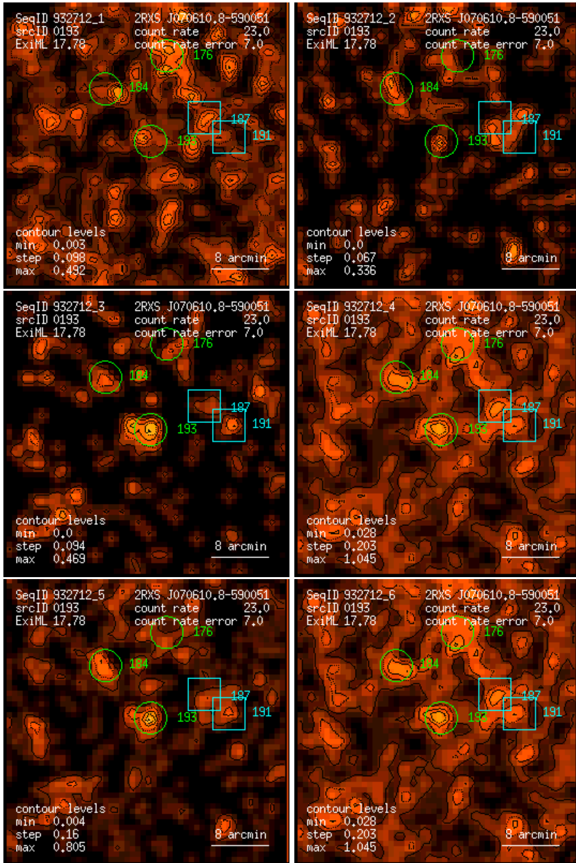
Figure 193: RASS 932712: detection 0193: band rate images, Gaussian filter: (1) PSPC channels 11 – 41, (2) 52 – 90, (3) 91 – 201, (4) 11 – 235, (5) 52 – 201, (6) 11 – 201. Broad band rates in counts/ks. Band rate contour levels in counts/ks/arcmin 2 .
