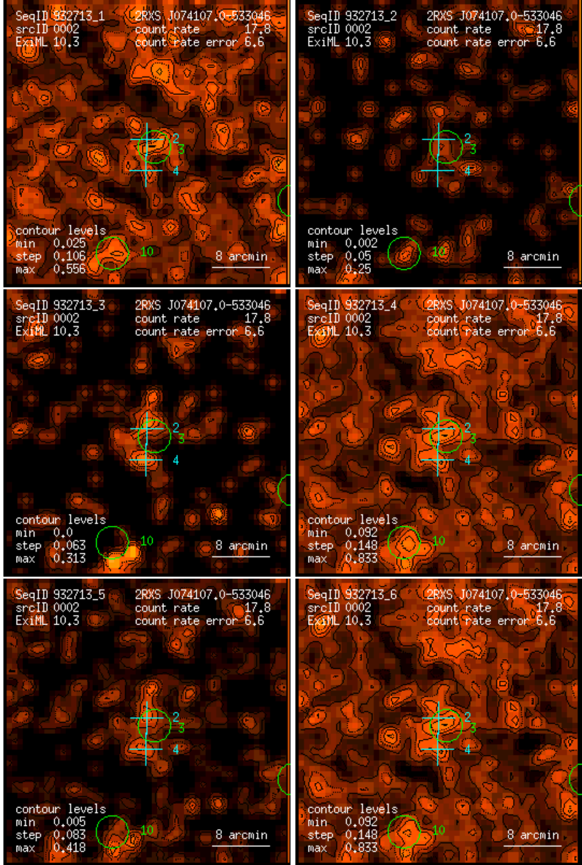
Figure 2: RASS 932713: detection 0002: band rate images, Gaussian filter: (1) PSPC channels 11 – 41, (2) 52 – 90, (3) 91 – 201, (4) 11 – 235, (5) 52 – 201, (6) 11 – 201. Broad band rates in counts/ks. Band rate contour levels in counts/ks/arcmin 2 .
