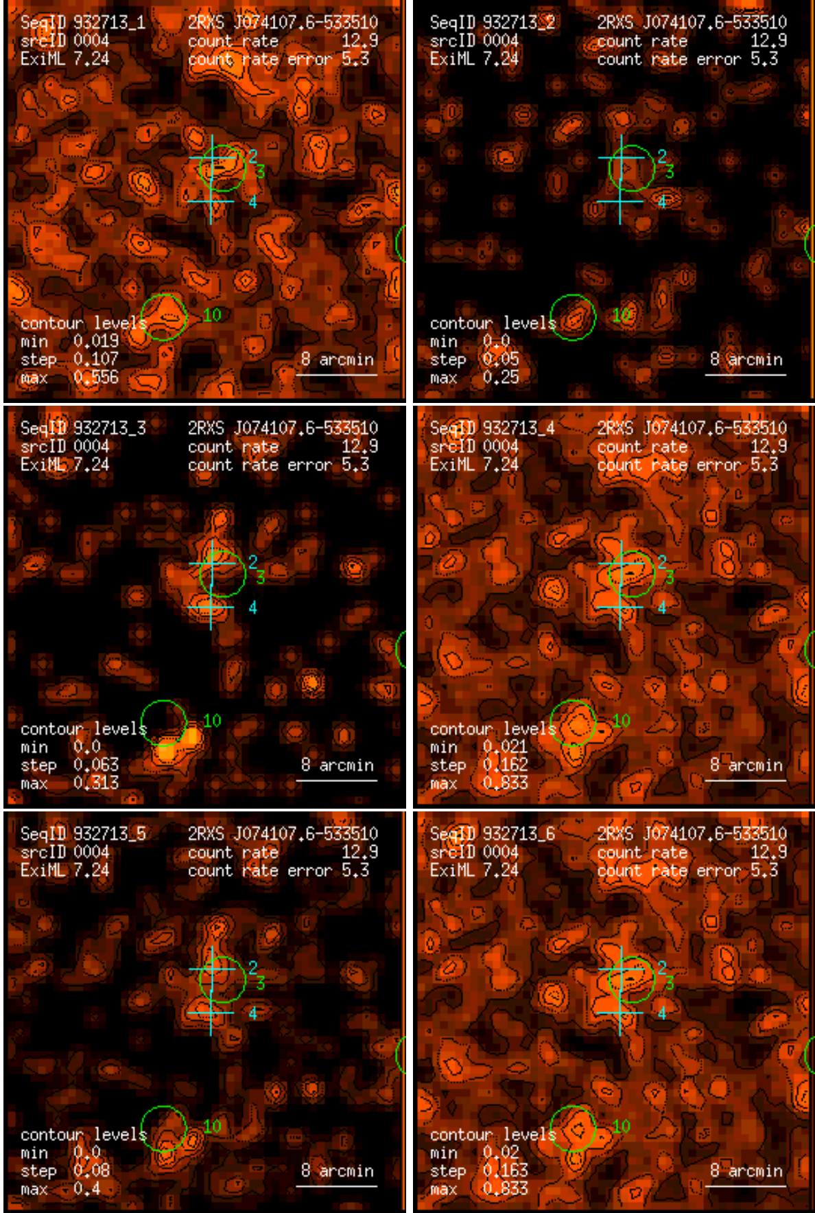
Figure 4: RASS 932713: detection 0004: band rate images, Gaussian filter: (1) PSPC channels 11 – 41, (2) 52 – 90, (3) 91 – 201, (4) 11 – 235, (5) 52 – 201, (6) 11 – 201. Broad band rates in counts/ks. Band rate contour levels in counts/ks/arcmin 2 .
