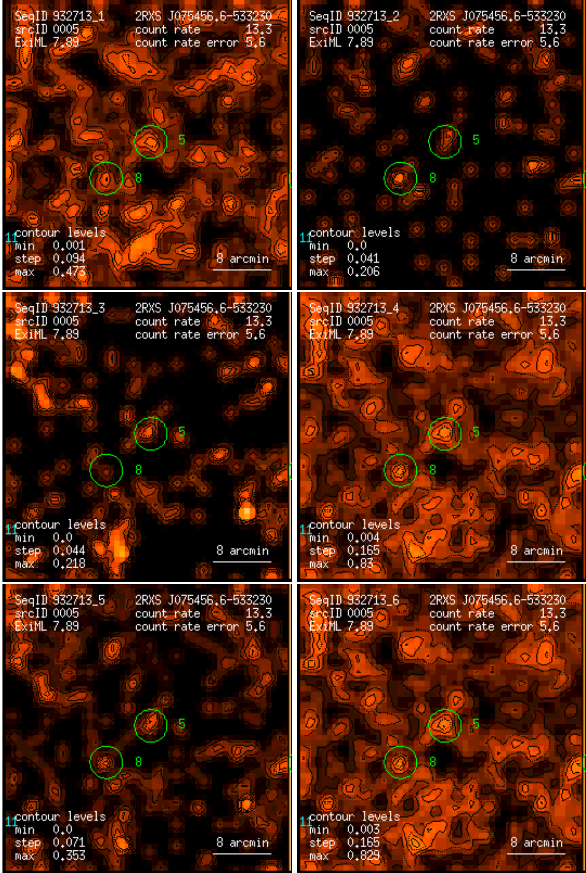
Figure 5: RASS 932713: detection 0005: band rate images, Gaussian filter: (1) PSPC channels 11 – 41, (2) 52 – 90, (3) 91 – 201, (4) 11 – 235, (5) 52 – 201, (6) 11 – 201. Broad band rates in counts/ks. Band rate contour levels in counts/ks/arcmin 2 .
