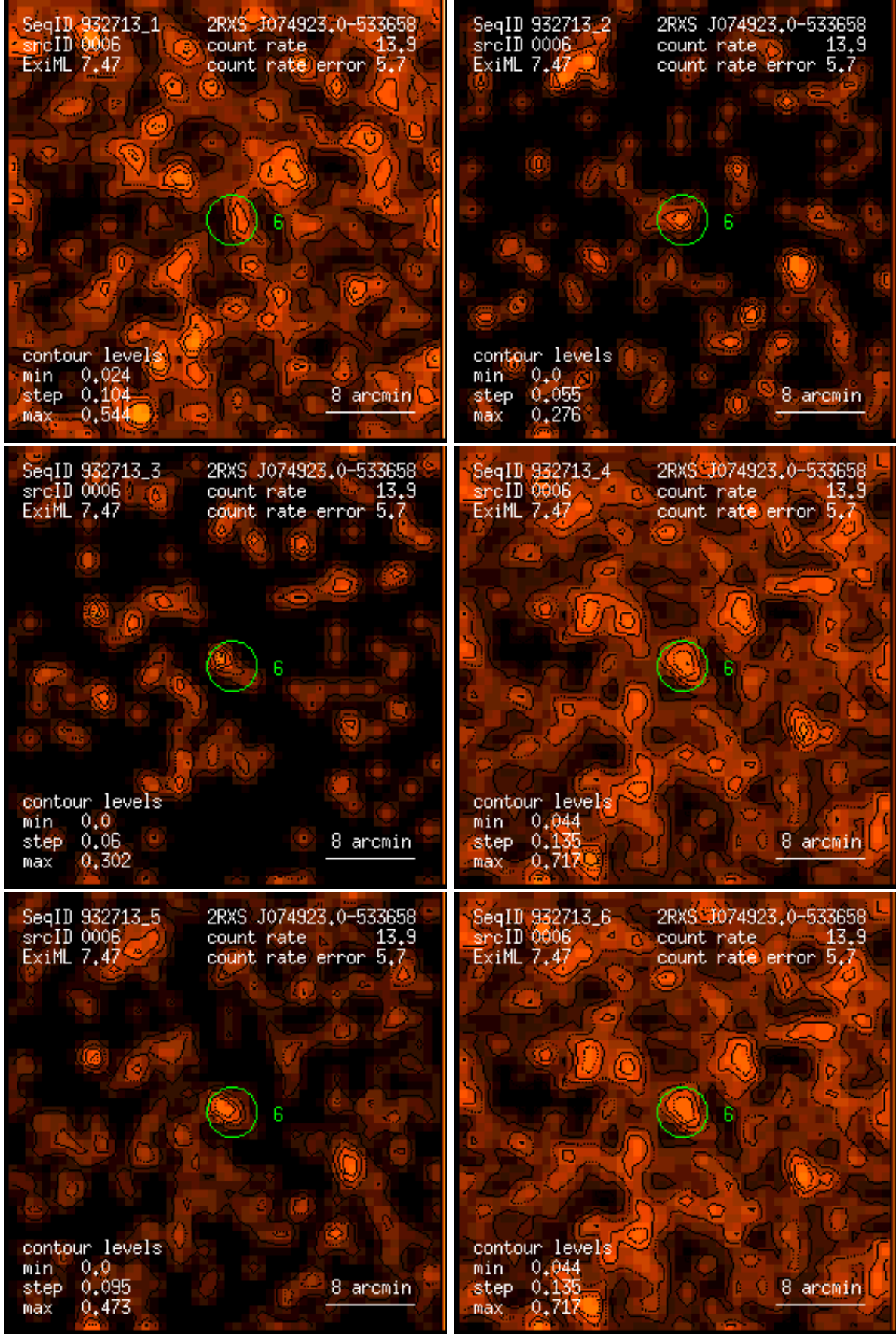
Figure 6: RASS 932713: detection 0006: band rate images, Gaussian filter: (1) PSPC channels 11 – 41, (2) 52 – 90, (3) 91 – 201, (4) 11 – 235, (5) 52 – 201, (6) 11 – 201. Broad band rates in counts/ks. Band rate contour levels in counts/ks/arcmin 2 .
