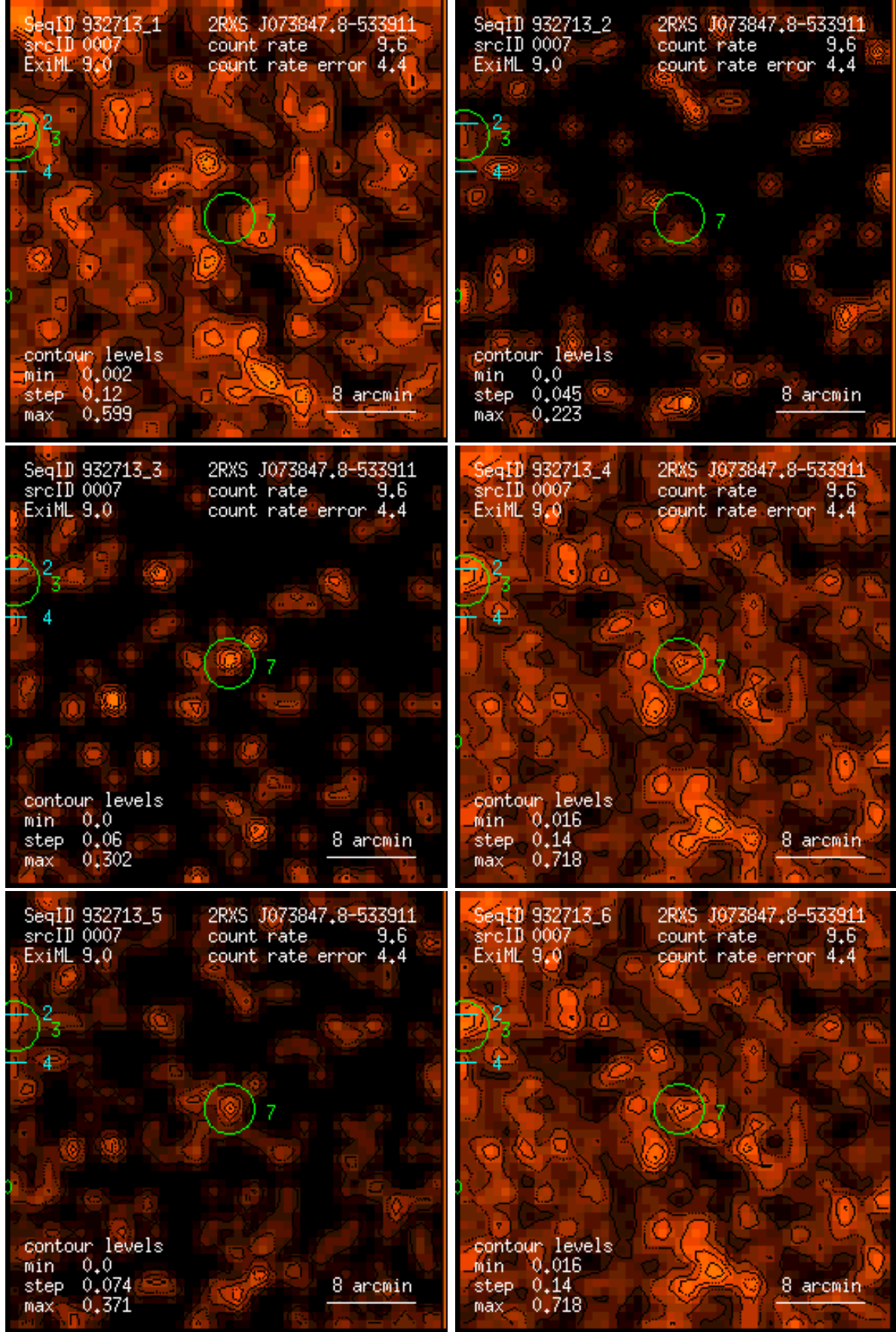
Figure 7: RASS 932713: detection 0007: band rate images, Gaussian filter: (1) PSPC channels 11 – 41, (2) 52 – 90, (3) 91 – 201, (4) 11 – 235, (5) 52 – 201, (6) 11 – 201. Broad band rates in counts/ks. Band rate contour levels in counts/ks/arcmin 2 .
