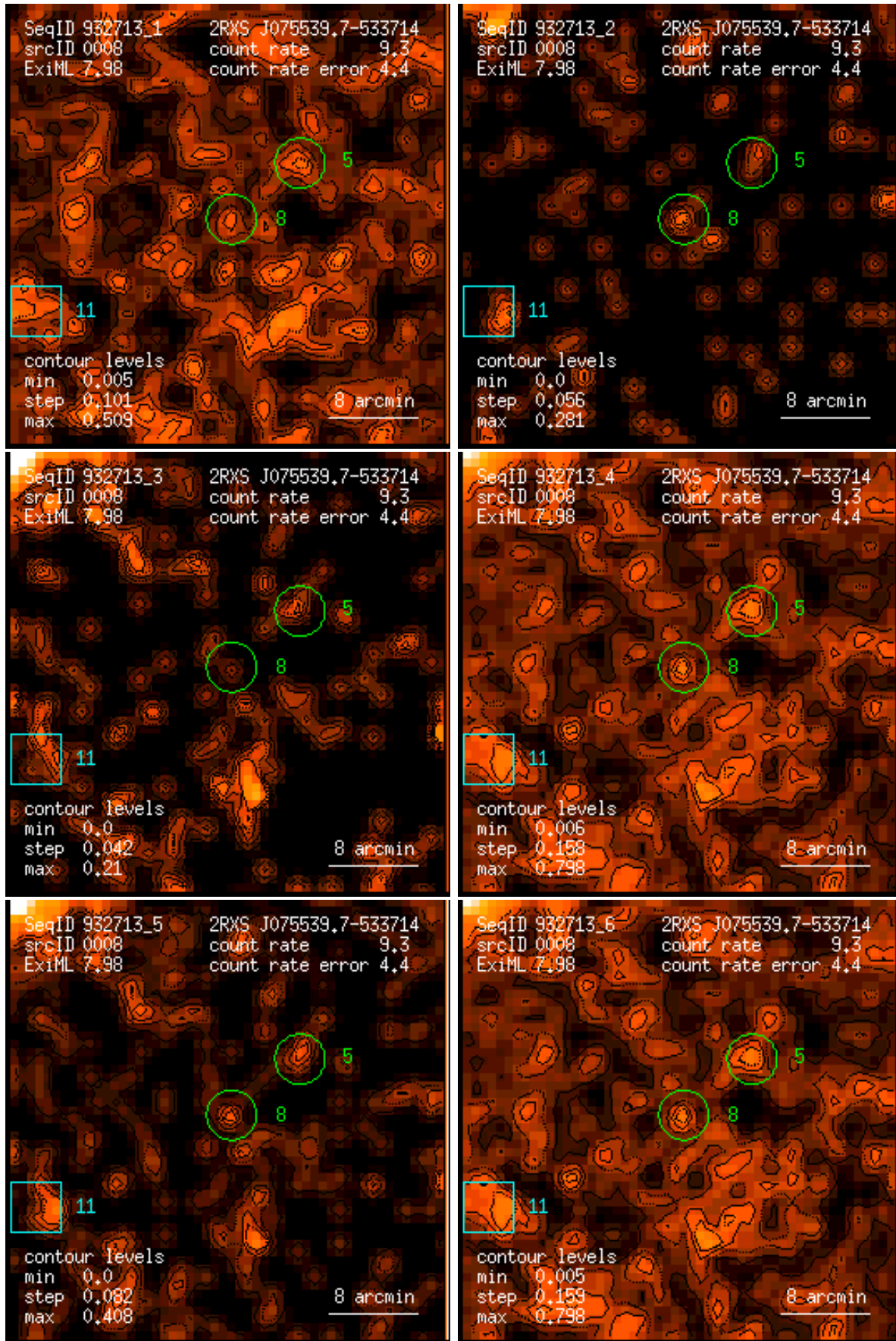
Figure 8: RASS 932713: detection 0008: band rate images, Gaussian filter: (1) PSPC channels 11 – 41, (2) 52 – 90, (3) 91 – 201, (4) 11 – 235, (5) 52 – 201, (6) 11 – 201. Broad band rates in counts/ks. Band rate contour levels in counts/ks/arcmin 2 .
