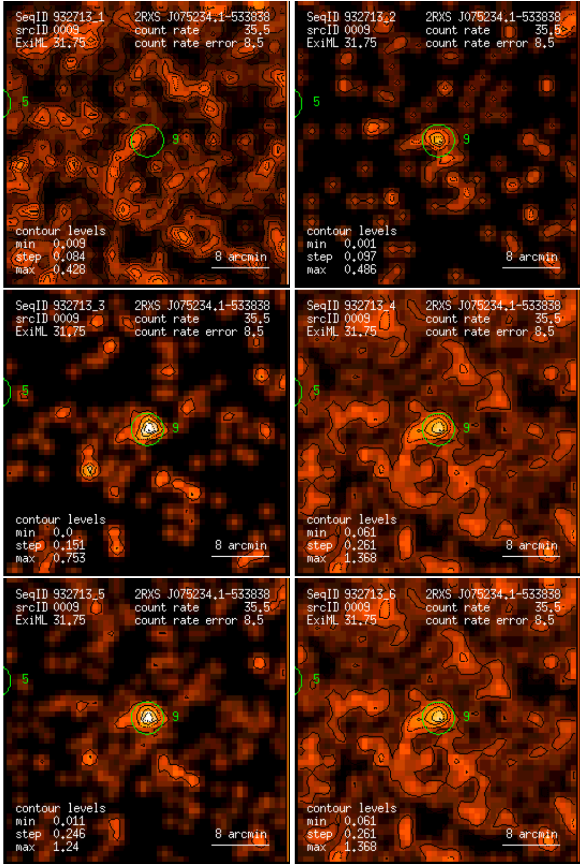
Figure 9: RASS 932713: detection 0009: band rate images, Gaussian filter: (1) PSPC channels 11 – 41, (2) 52 – 90, (3) 91 – 201, (4) 11 – 235, (5) 52 – 201, (6) 11 – 201. Broad band rates in counts/ks. Band rate contour levels in counts/ks/arcmin 2 .
