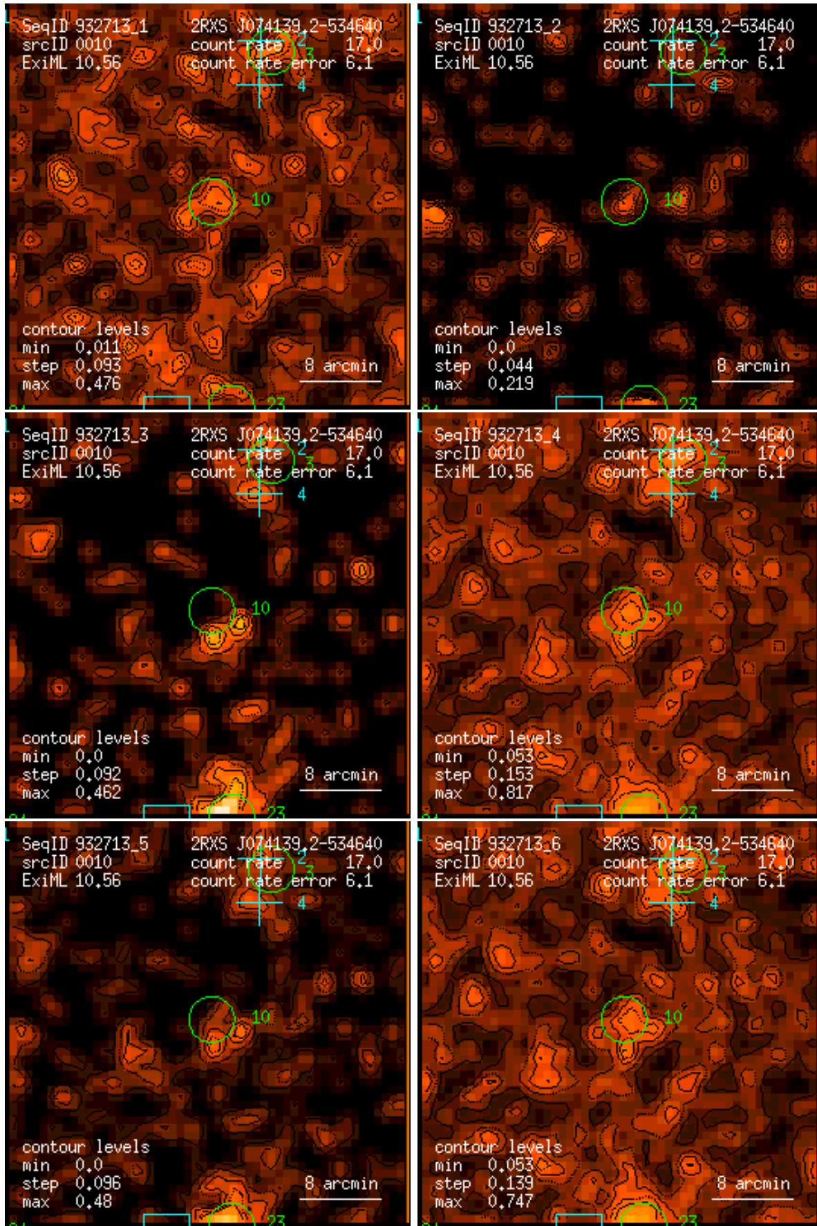
Figure 10: RASS 932713: detection 0010: band rate images, Gaussian filter: (1) PSPC channels 11 – 41, (2) 52 – 90, (3) 91 – 201, (4) 11 – 235, (5) 52 – 201, (6) 11 – 201. Broad band rates in counts/ks. Band rate contour levels in counts/ks/arcmin 2 .
