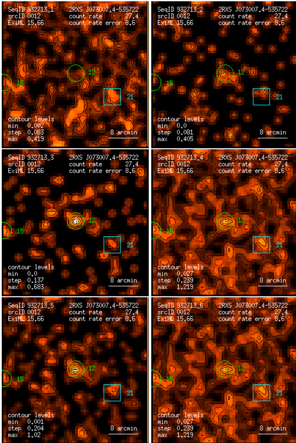
Figure 12: RASS 932713: detection 0012: band rate images, Gaussian filter: (1) PSPC channels 11 – 41, (2) 52 – 90, (3) 91 – 201, (4) 11 – 235, (5) 52 – 201, (6) 11 – 201. Broad band rates in counts/ks. Band rate contour levels in counts/ks/arcmin 2 .
