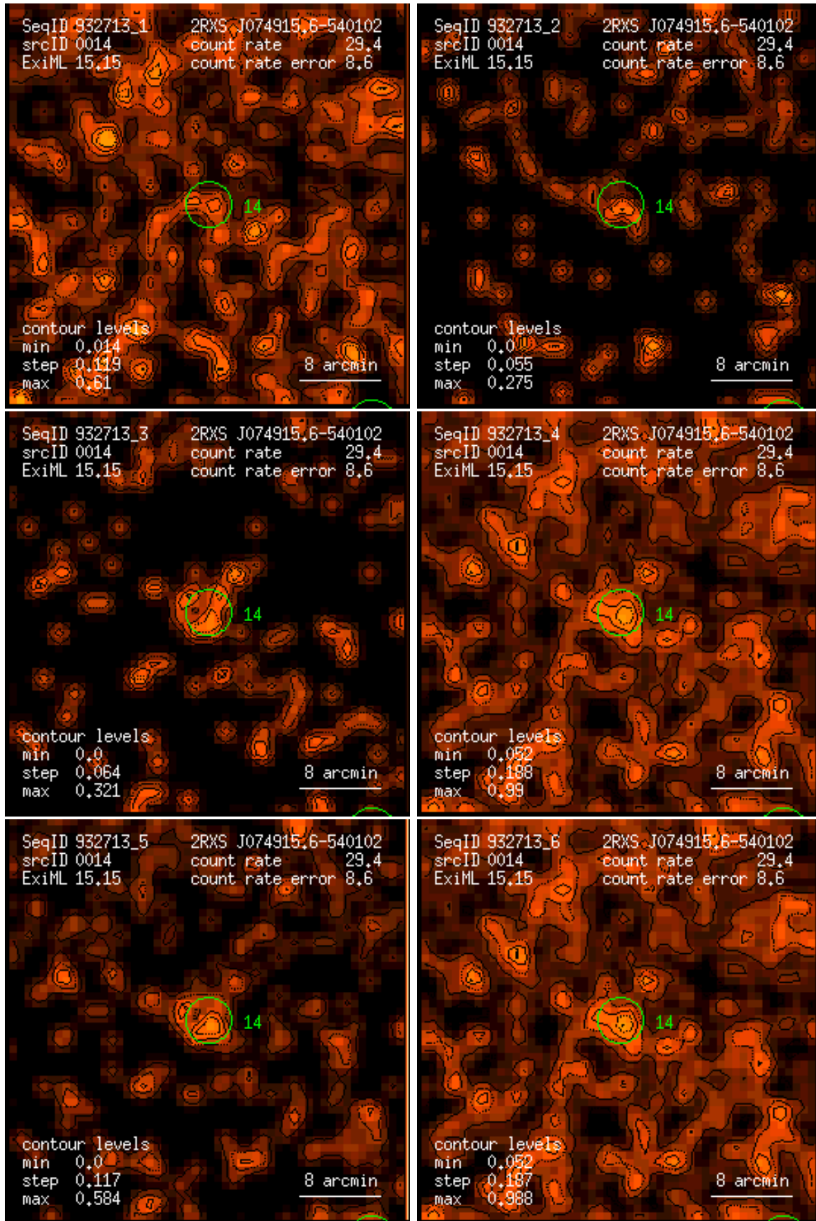
Figure 14: RASS 932713: detection 0014: band rate images, Gaussian filter: (1) PSPC channels 11 – 41, (2) 52 – 90, (3) 91 – 201, (4) 11 – 235, (5) 52 – 201, (6) 11 – 201. Broad band rates in counts/ks. Band rate contour levels in counts/ks/arcmin 2 .
