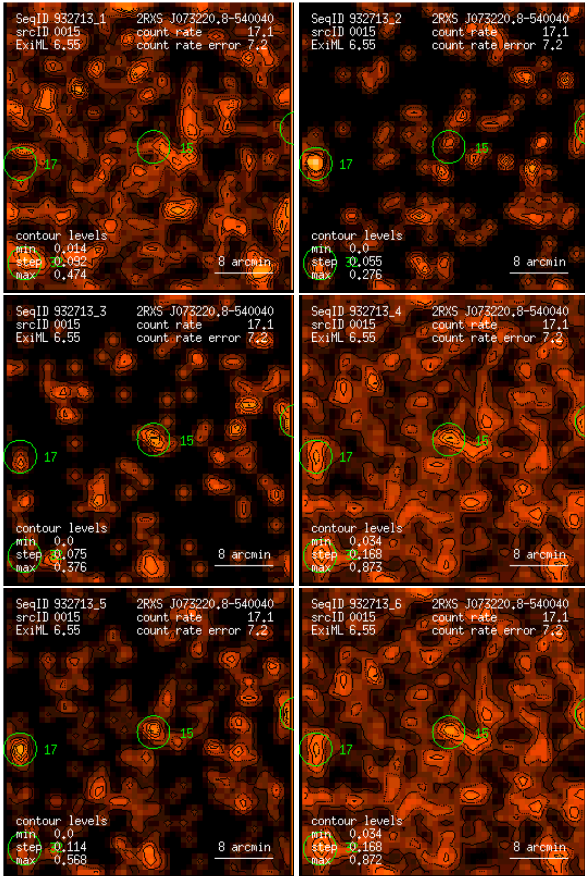
Figure 15: RASS 932713: detection 0015: band rate images, Gaussian filter: (1) PSPC channels 11 – 41, (2) 52 – 90, (3) 91 – 201, (4) 11 – 235, (5) 52 – 201, (6) 11 – 201. Broad band rates in counts/ks. Band rate contour levels in counts/ks/arcmin 2 .
