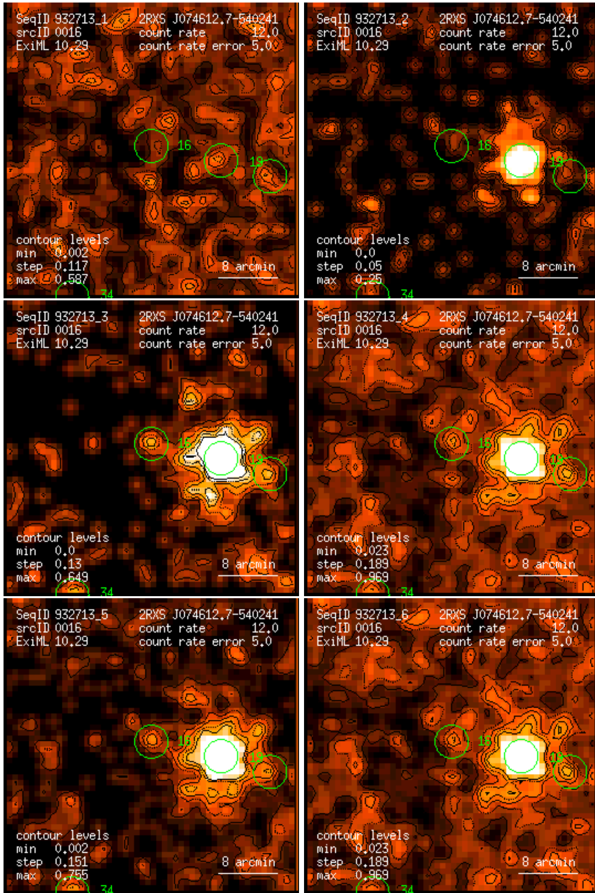
Figure 16: RASS 932713: detection 0016: band rate images, Gaussian filter: (1) PSPC channels 11 – 41, (2) 52 – 90, (3) 91 – 201, (4) 11 – 235, (5) 52 – 201, (6) 11 – 201. Broad band rates in counts/ks. Band rate contour levels in counts/ks/arcmin 2 .
