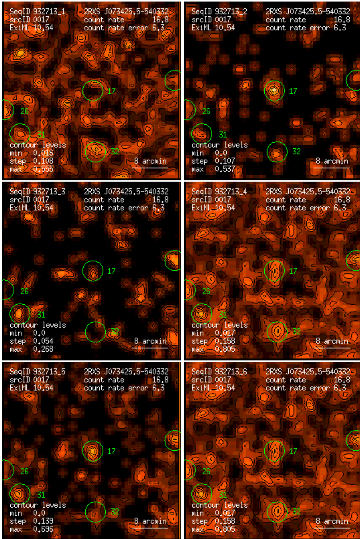
Figure 17: RASS 932713: detection 0017: band rate images, Gaussian filter: (1) PSPC channels 11 – 41, (2) 52 – 90, (3) 91 – 201, (4) 11 – 235, (5) 52 – 201, (6) 11 – 201. Broad band rates in counts/ks. Band rate contour levels in counts/ks/arcmin 2 .
