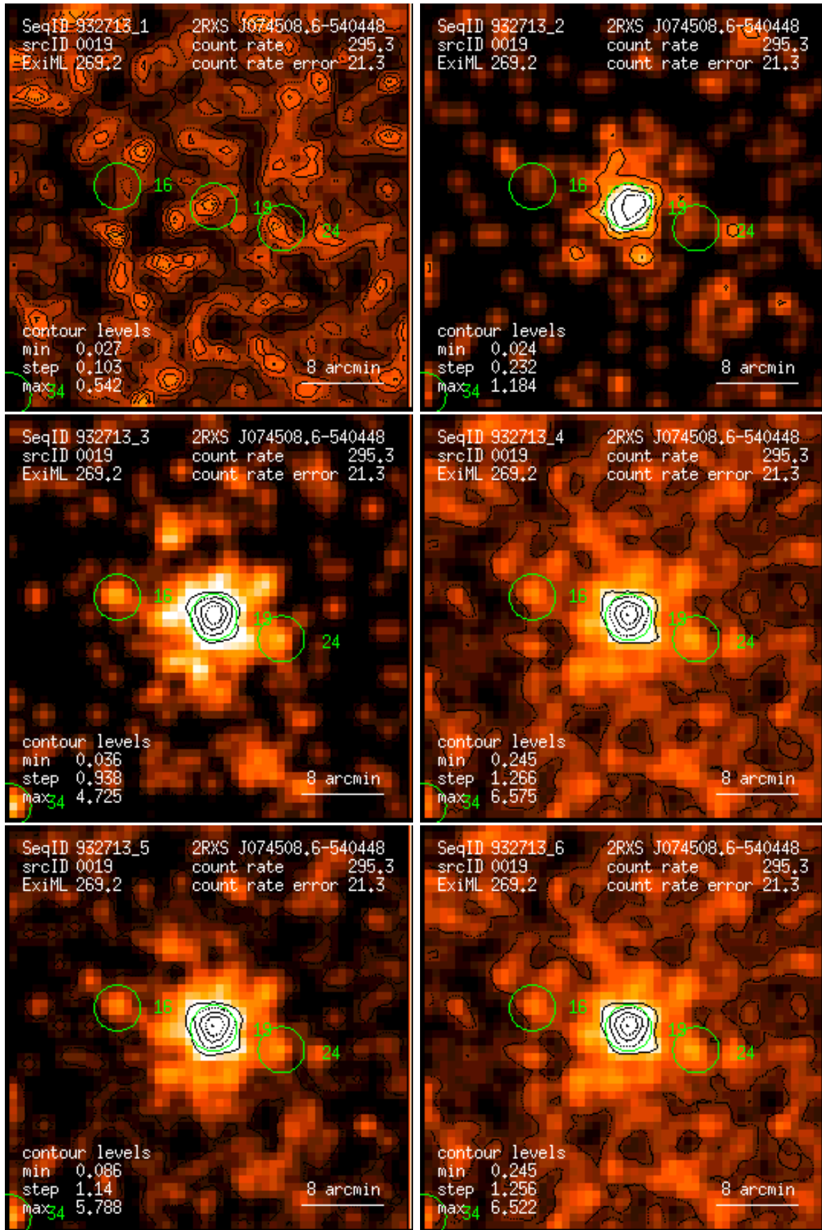
Figure 19: RASS 932713: detection 0019: band rate images, Gaussian filter: (1) PSPC channels 11 – 41, (2) 52 – 90, (3) 91 – 201, (4) 11 – 235, (5) 52 – 201, (6) 11 – 201. Broad band rates in counts/ks. Band rate contour levels in counts/ks/arcmin 2 .
