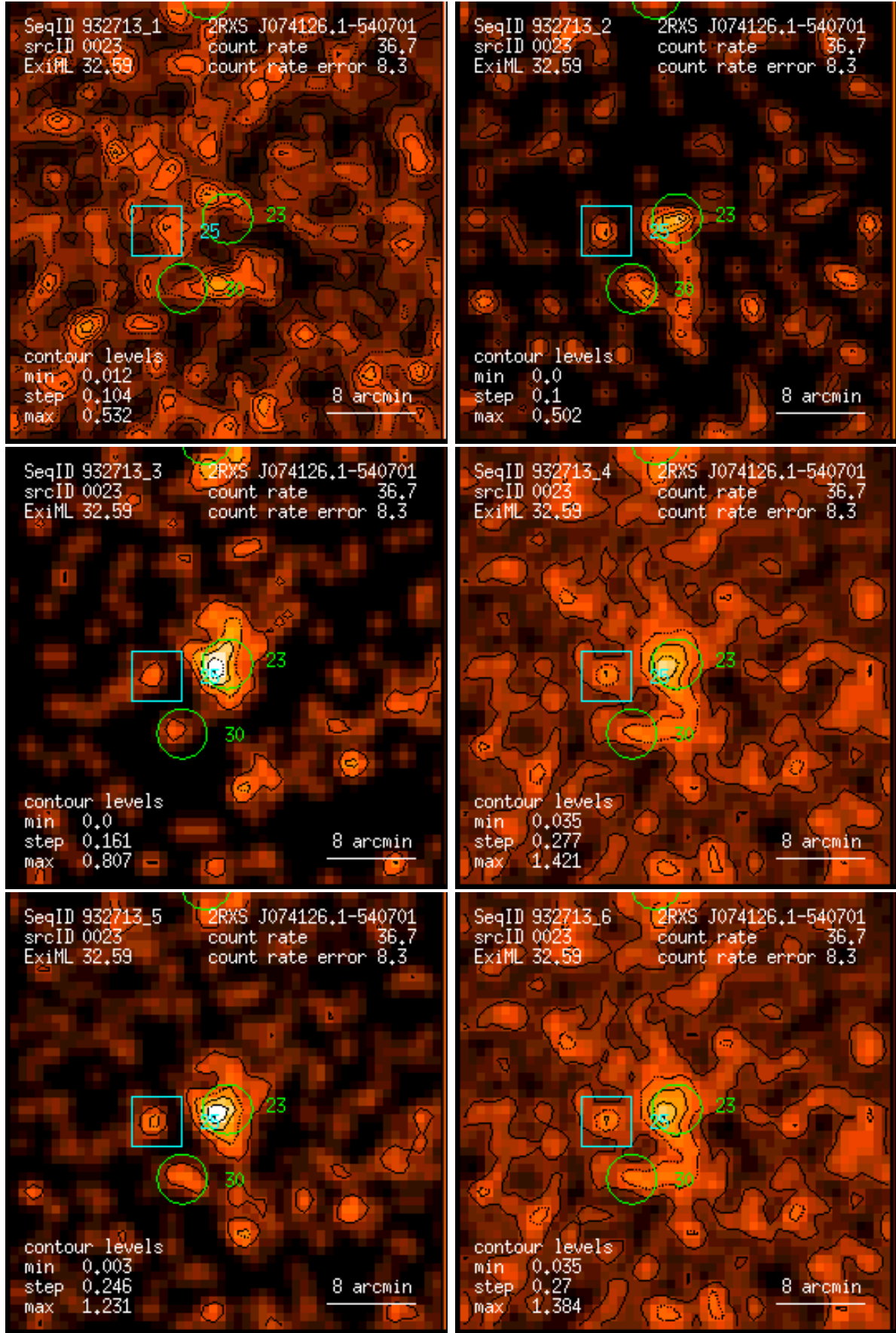
Figure 23: RASS 932713: detection 0023: band rate images, Gaussian filter: (1) PSPC channels 11 – 41, (2) 52 – 90, (3) 91 – 201, (4) 11 – 235, (5) 52 – 201, (6) 11 – 201. Broad band rates in counts/ks. Band rate contour levels in counts/ks/arcmin 2 .
