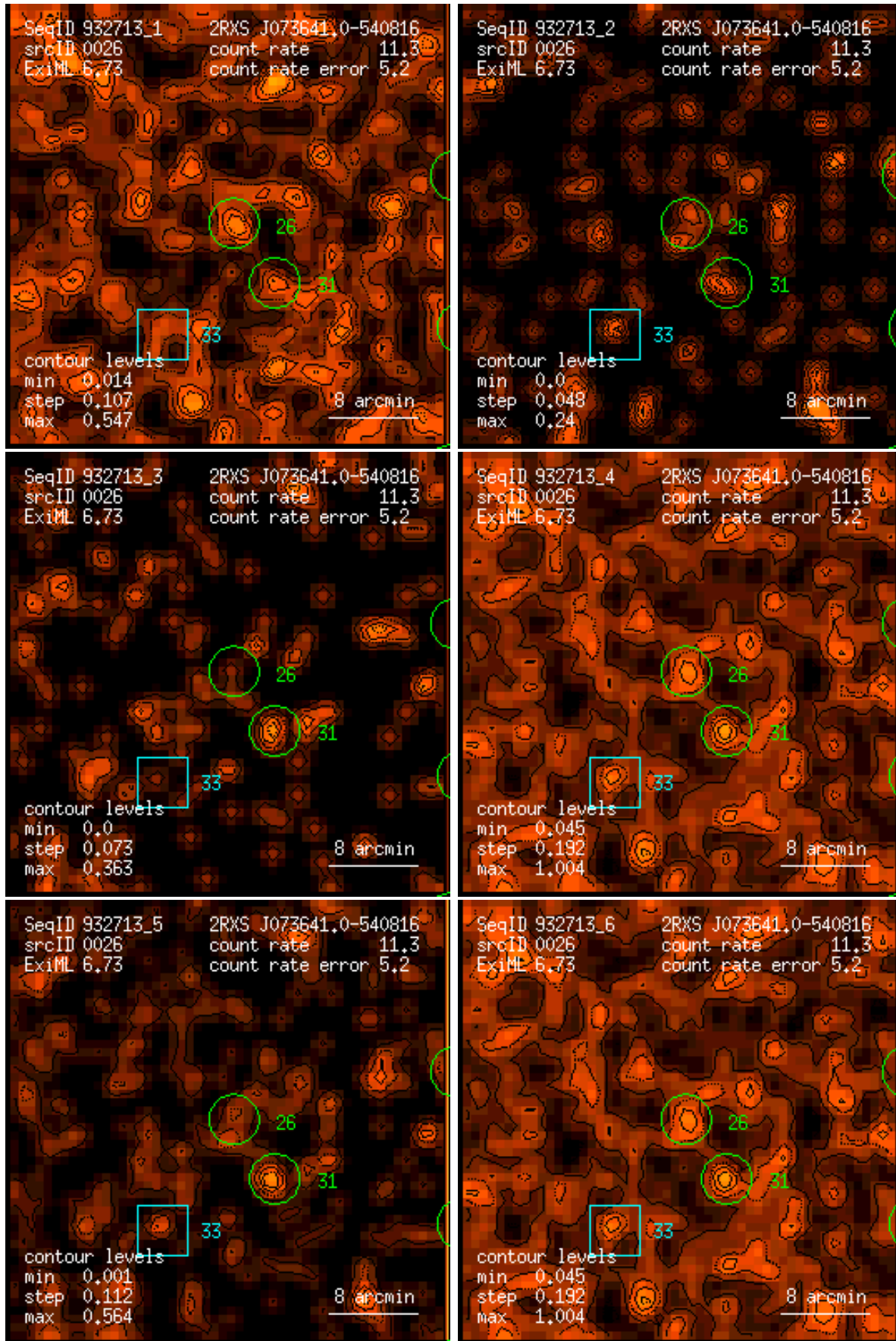
Figure 26: RASS 932713: detection 0026: band rate images, Gaussian filter: (1) PSPC channels 11 – 41, (2) 52 – 90, (3) 91 – 201, (4) 11 – 235, (5) 52 – 201, (6) 11 – 201. Broad band rates in counts/ks. Band rate contour levels in counts/ks/arcmin 2 .
