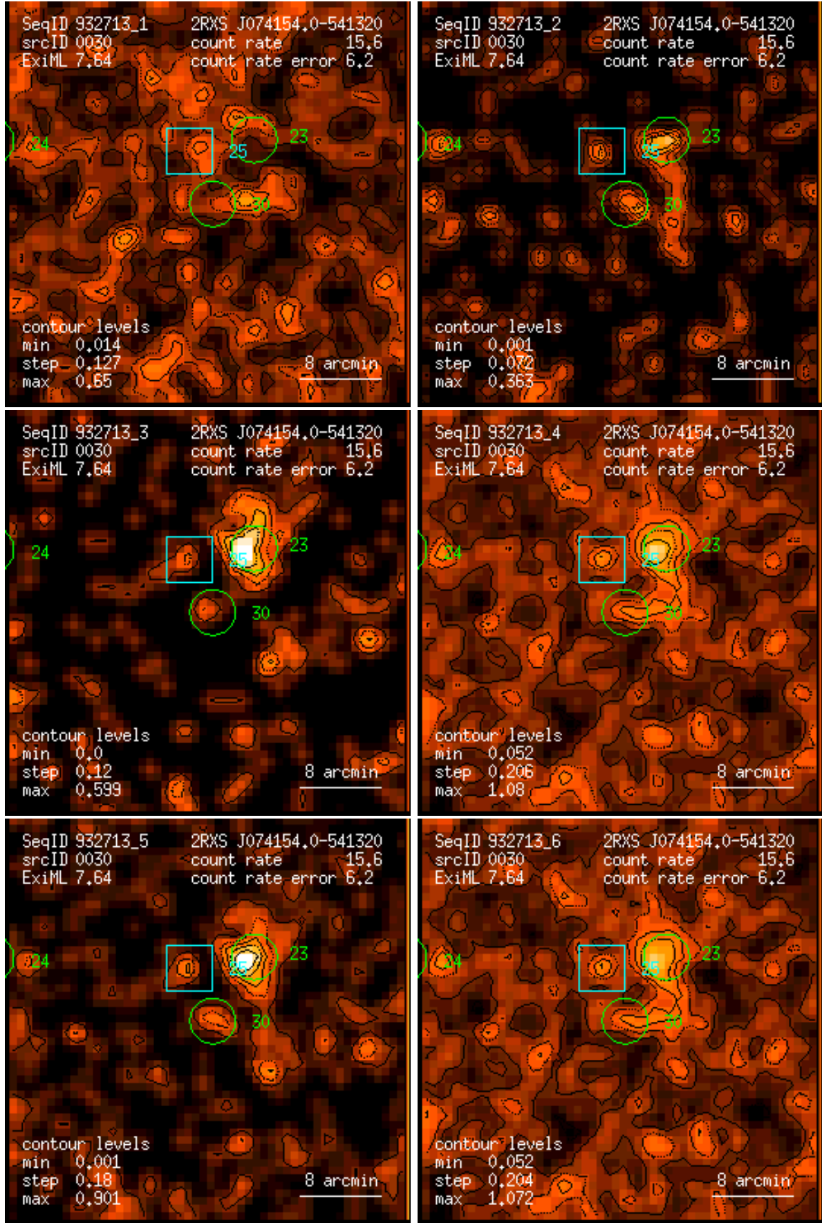
Figure 30: RASS 932713: detection 0030: band rate images, Gaussian filter: (1) PSPC channels 11 – 41, (2) 52 – 90, (3) 91 – 201, (4) 11 – 235, (5) 52 – 201, (6) 11 – 201. Broad band rates in counts/ks. Band rate contour levels in counts/ks/arcmin 2 .
