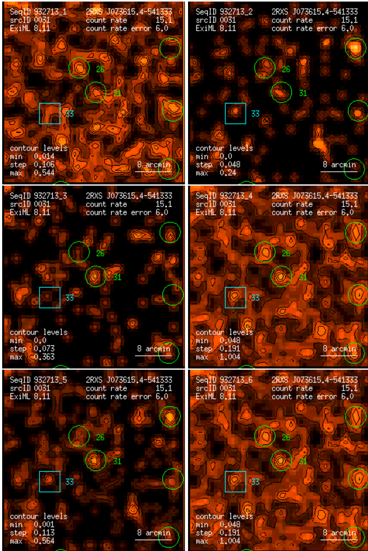
Figure 31: RASS 932713: detection 0031: band rate images, Gaussian filter: (1) PSPC channels 11 – 41, (2) 52 – 90, (3) 91 – 201, (4) 11 – 235, (5) 52 – 201, (6) 11 – 201. Broad band rates in counts/ks. Band rate contour levels in counts/ks/arcmin 2 .
