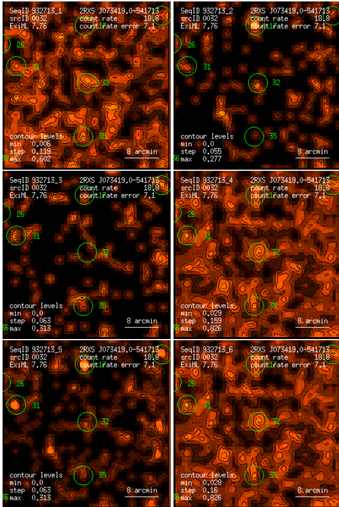
Figure 32: RASS 932713: detection 0032: band rate images, Gaussian filter: (1) PSPC channels 11 – 41, (2) 52 – 90, (3) 91 – 201, (4) 11 – 235, (5) 52 – 201, (6) 11 – 201. Broad band rates in counts/ks. Band rate contour levels in counts/ks/arcmin 2 .
