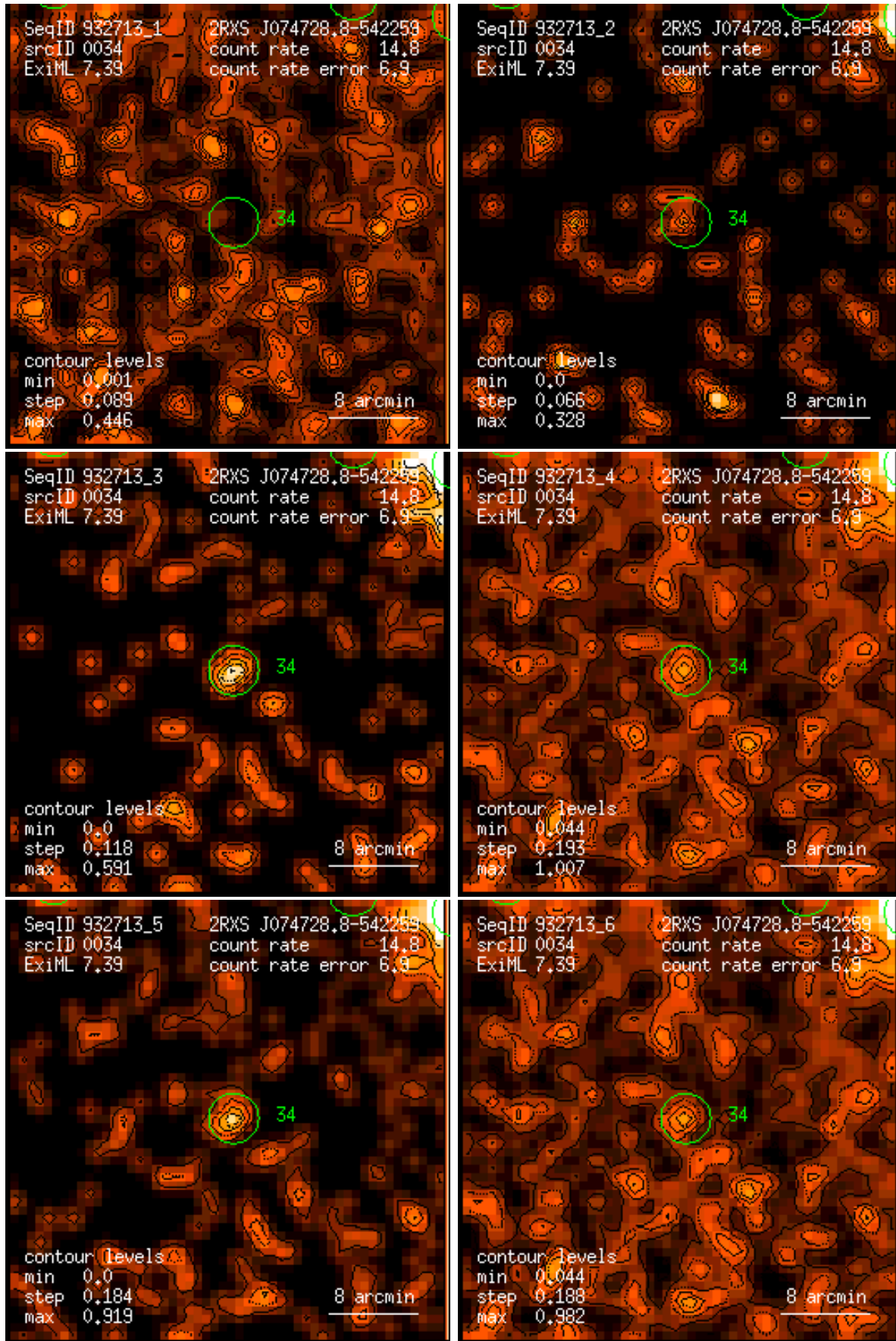
Figure 34: RASS 932713: detection 0034: band rate images, Gaussian filter: (1) PSPC channels 11 – 41, (2) 52 – 90, (3) 91 – 201, (4) 11 – 235, (5) 52 – 201, (6) 11 – 201. Broad band rates in counts/ks. Band rate contour levels in counts/ks/arcmin 2 .
