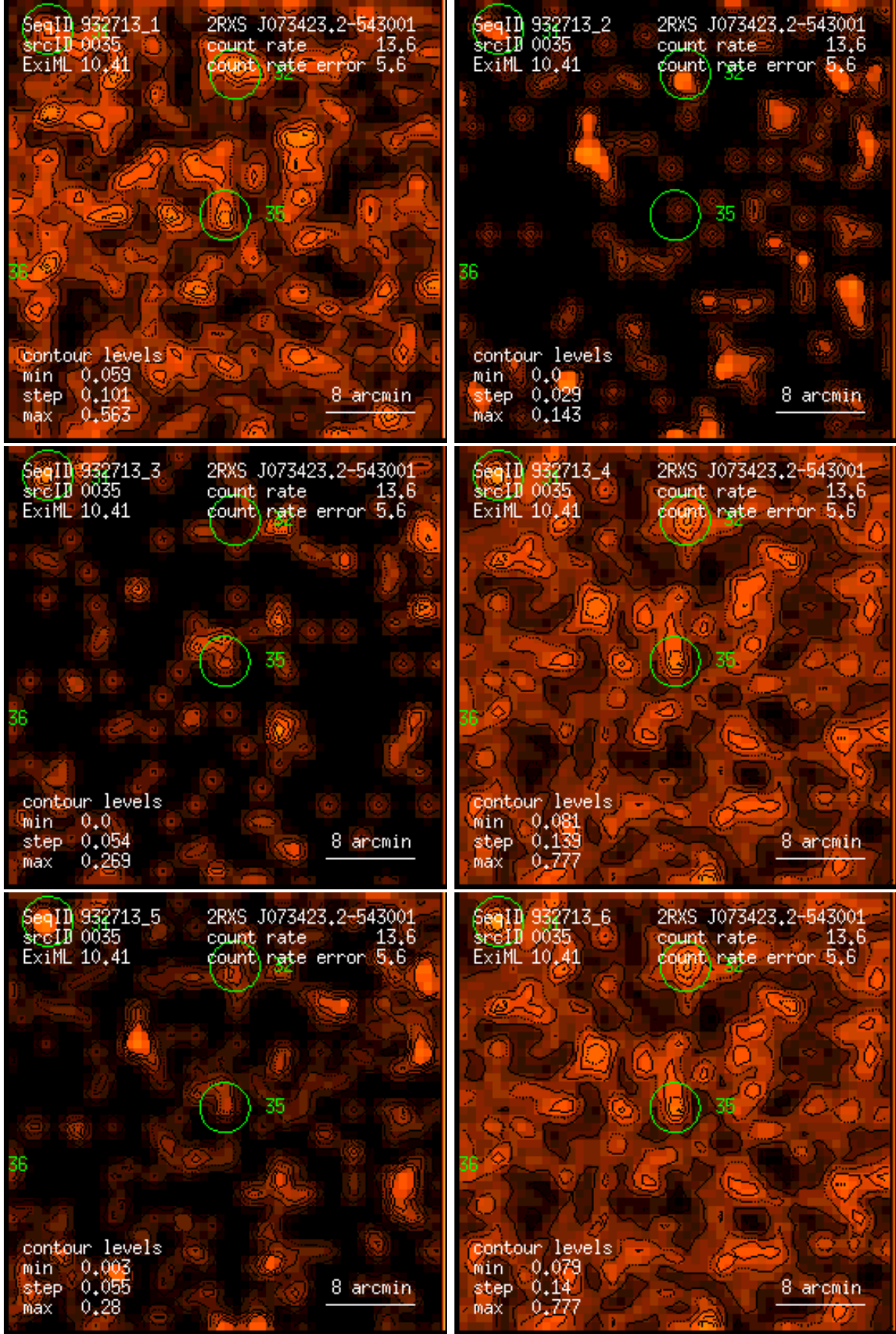
Figure 35: RASS 932713: detection 0035: band rate images, Gaussian filter: (1) PSPC channels 11 – 41, (2) 52 – 90, (3) 91 – 201, (4) 11 – 235, (5) 52 – 201, (6) 11 – 201. Broad band rates in counts/ks. Band rate contour levels in counts/ks/arcmin 2 .
