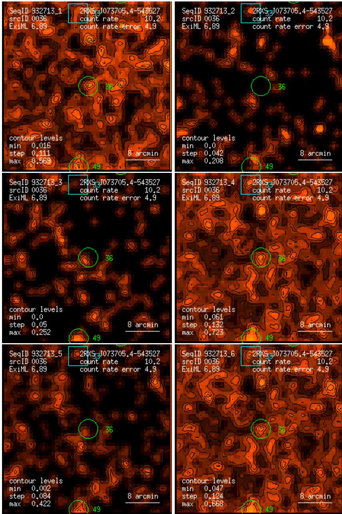
Figure 36: RASS 932713: detection 0036: band rate images, Gaussian filter: (1) PSPC channels 11 – 41, (2) 52 – 90, (3) 91 – 201, (4) 11 – 235, (5) 52 – 201, (6) 11 – 201. Broad band rates in counts/ks. Band rate contour levels in counts/ks/arcmin 2 .
