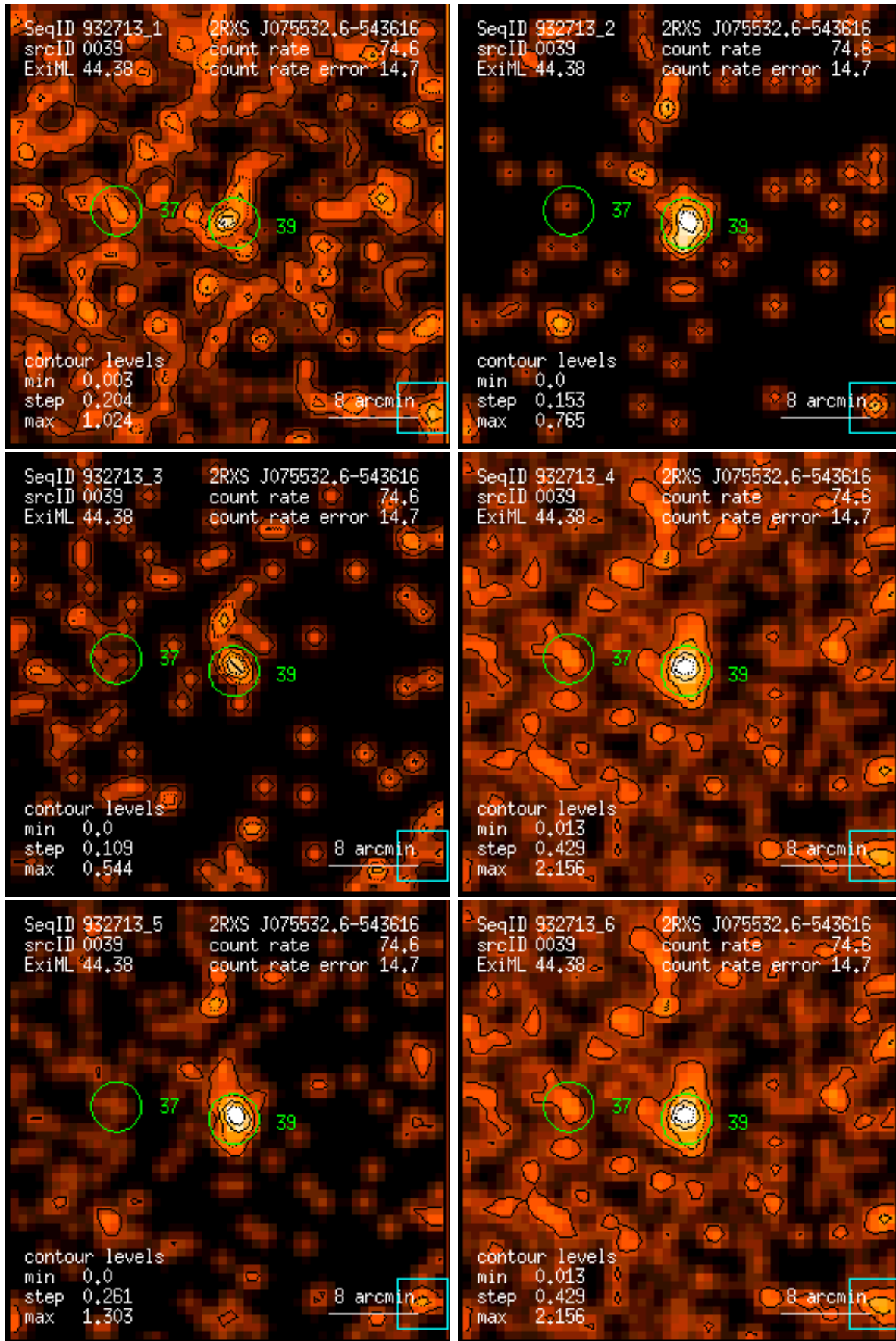
Figure 39: RASS 932713: detection 0039: band rate images, Gaussian filter: (1) PSPC channels 11 – 41, (2) 52 – 90, (3) 91 – 201, (4) 11 – 235, (5) 52 – 201, (6) 11 – 201. Broad band rates in counts/ks. Band rate contour levels in counts/ks/arcmin 2 .
