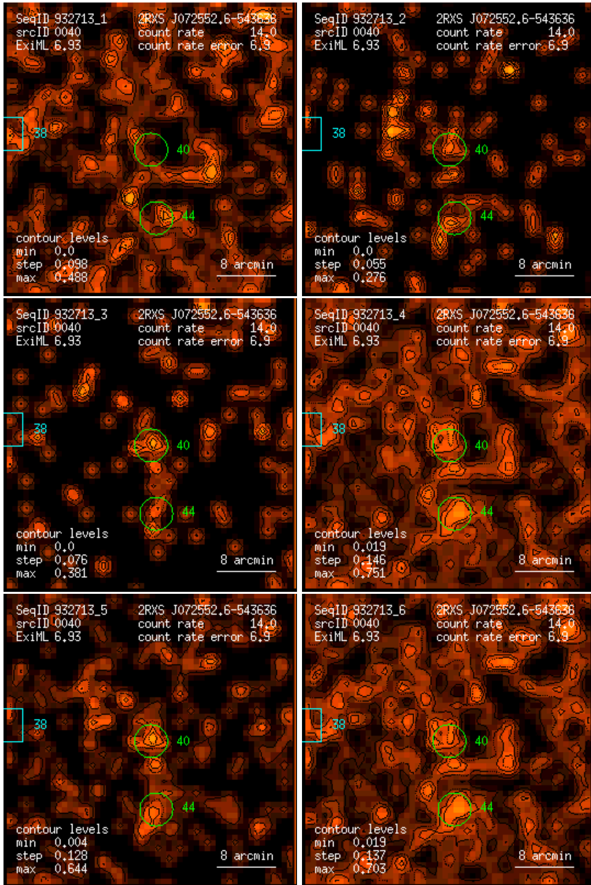
Figure 40: RASS 932713: detection 0040: band rate images, Gaussian filter: (1) PSPC channels 11 – 41, (2) 52 – 90, (3) 91 – 201, (4) 11 – 235, (5) 52 – 201, (6) 11 – 201. Broad band rates in counts/ks. Band rate contour levels in counts/ks/arcmin 2 .
