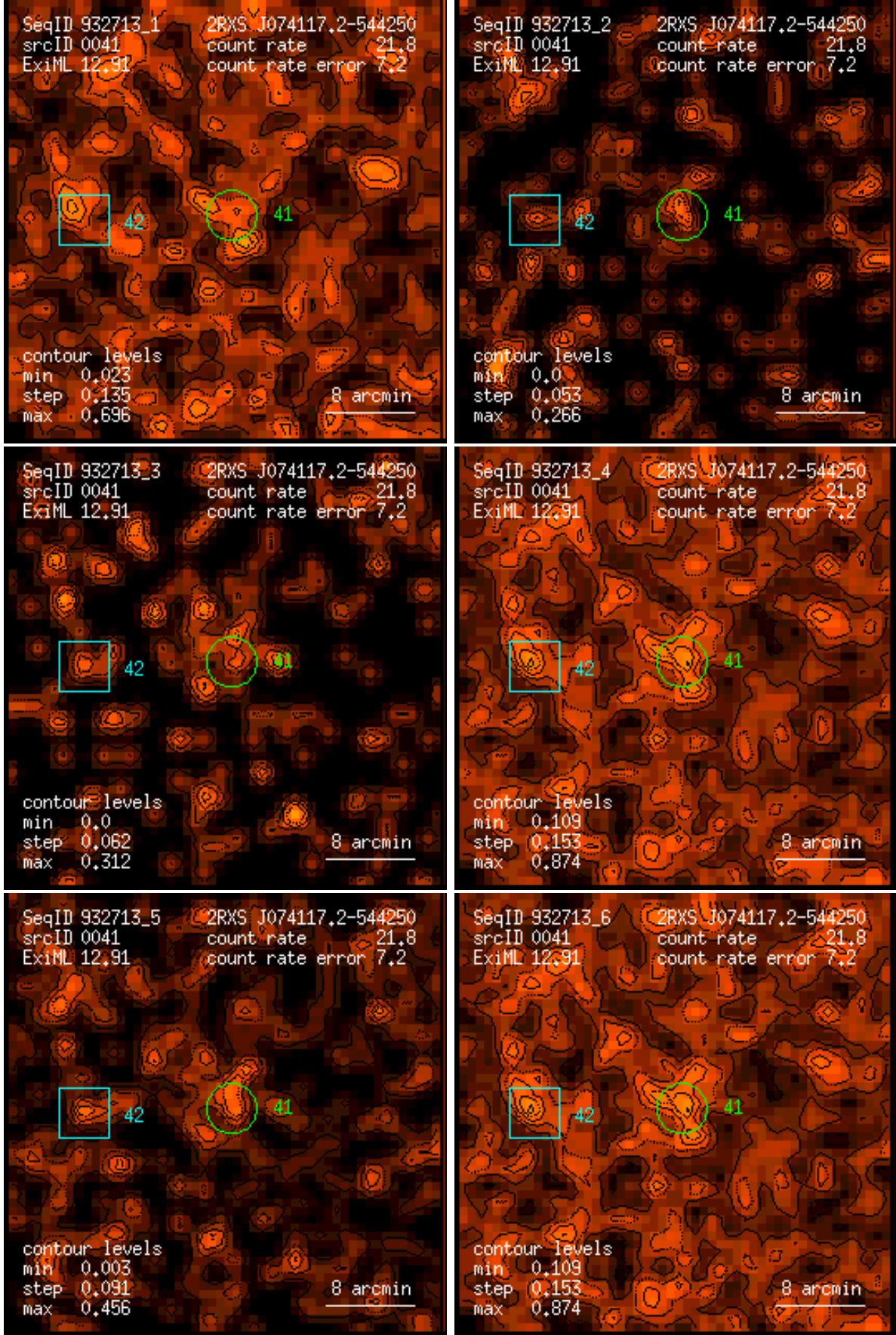
Figure 41: RASS 932713: detection 0041: band rate images, Gaussian filter: (1) PSPC channels 11 – 41, (2) 52 – 90, (3) 91 – 201, (4) 11 – 235, (5) 52 – 201, (6) 11 – 201. Broad band rates in counts/ks. Band rate contour levels in counts/ks/arcmin 2 .
