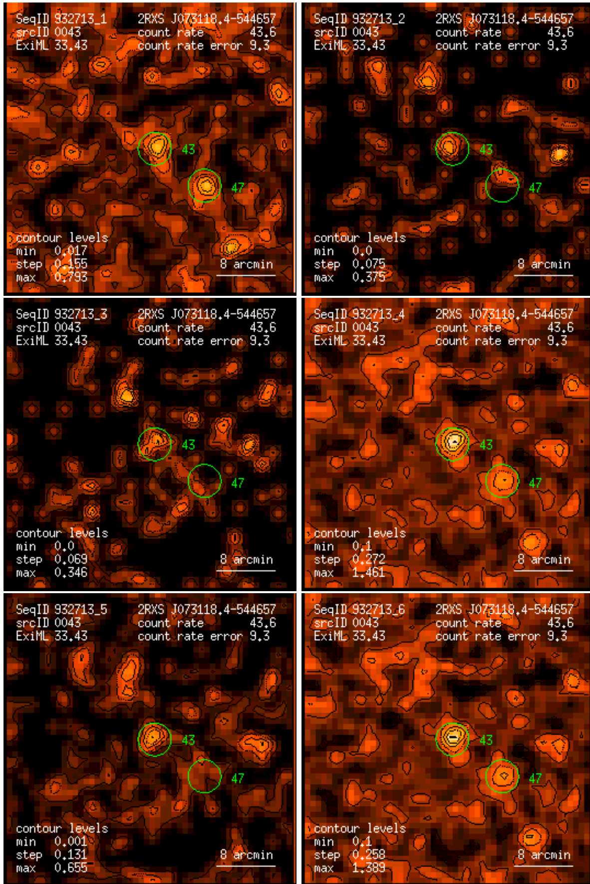
Figure 43: RASS 932713: detection 0043: band rate images, Gaussian filter: (1) PSPC channels 11 – 41, (2) 52 – 90, (3) 91 – 201, (4) 11 – 235, (5) 52 – 201, (6) 11 – 201. Broad band rates in counts/ks. Band rate contour levels in counts/ks/arcmin 2 .
