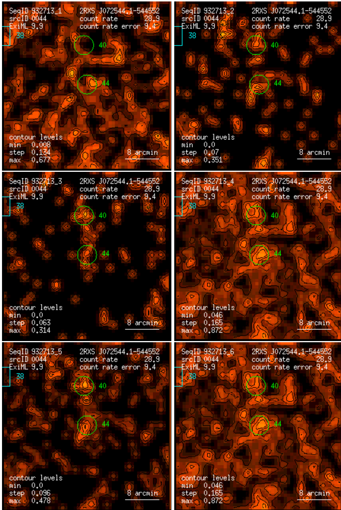
Figure 44: RASS 932713: detection 0044: band rate images, Gaussian filter: (1) PSPC channels 11 – 41, (2) 52 – 90, (3) 91 – 201, (4) 11 – 235, (5) 52 – 201, (6) 11 – 201. Broad band rates in counts/ks. Band rate contour levels in counts/ks/arcmin 2 .
