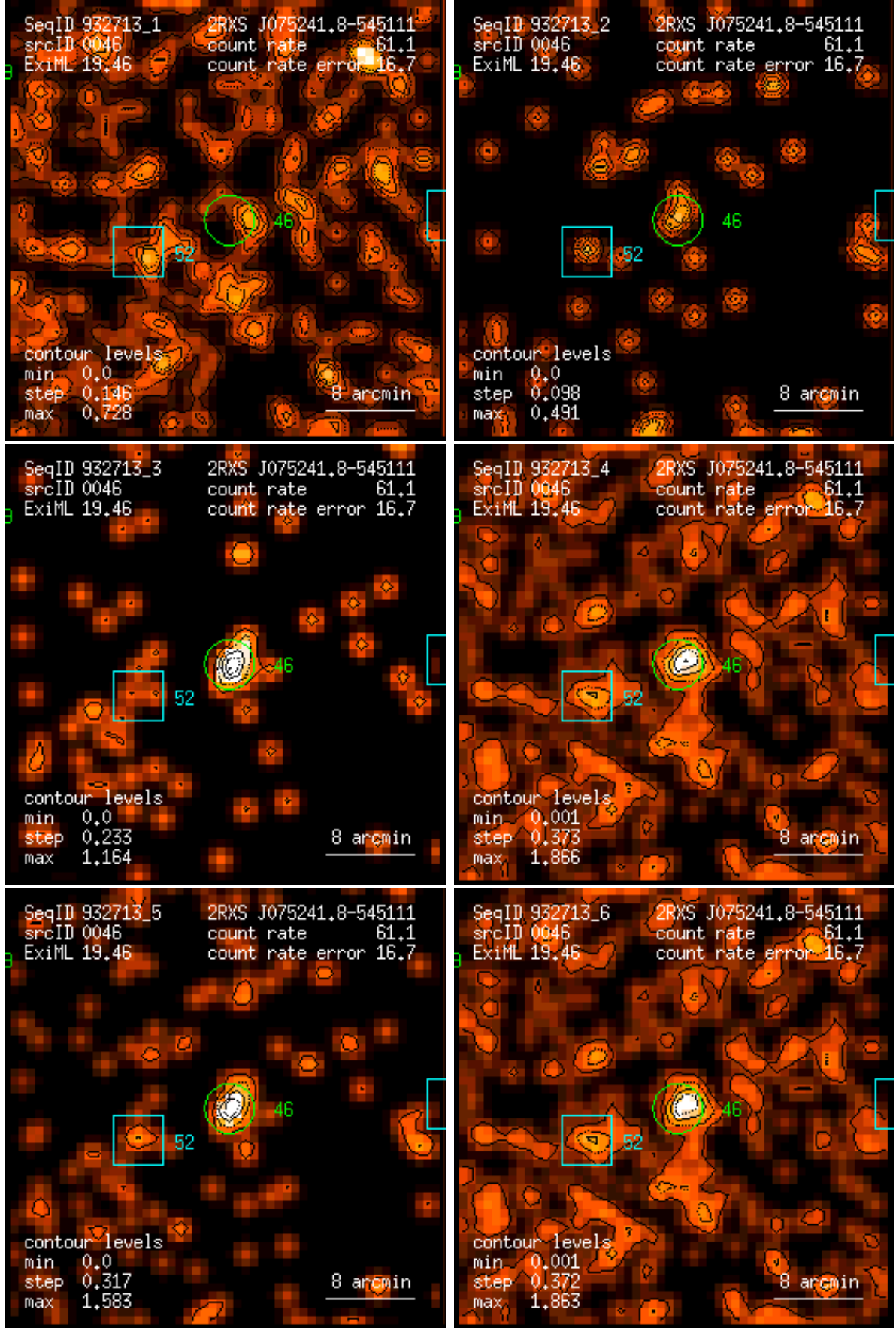
Figure 46: RASS 932713: detection 0046: band rate images, Gaussian filter: (1) PSPC channels 11 – 41, (2) 52 – 90, (3) 91 – 201, (4) 11 – 235, (5) 52 – 201, (6) 11 – 201. Broad band rates in counts/ks. Band rate contour levels in counts/ks/arcmin 2 .
