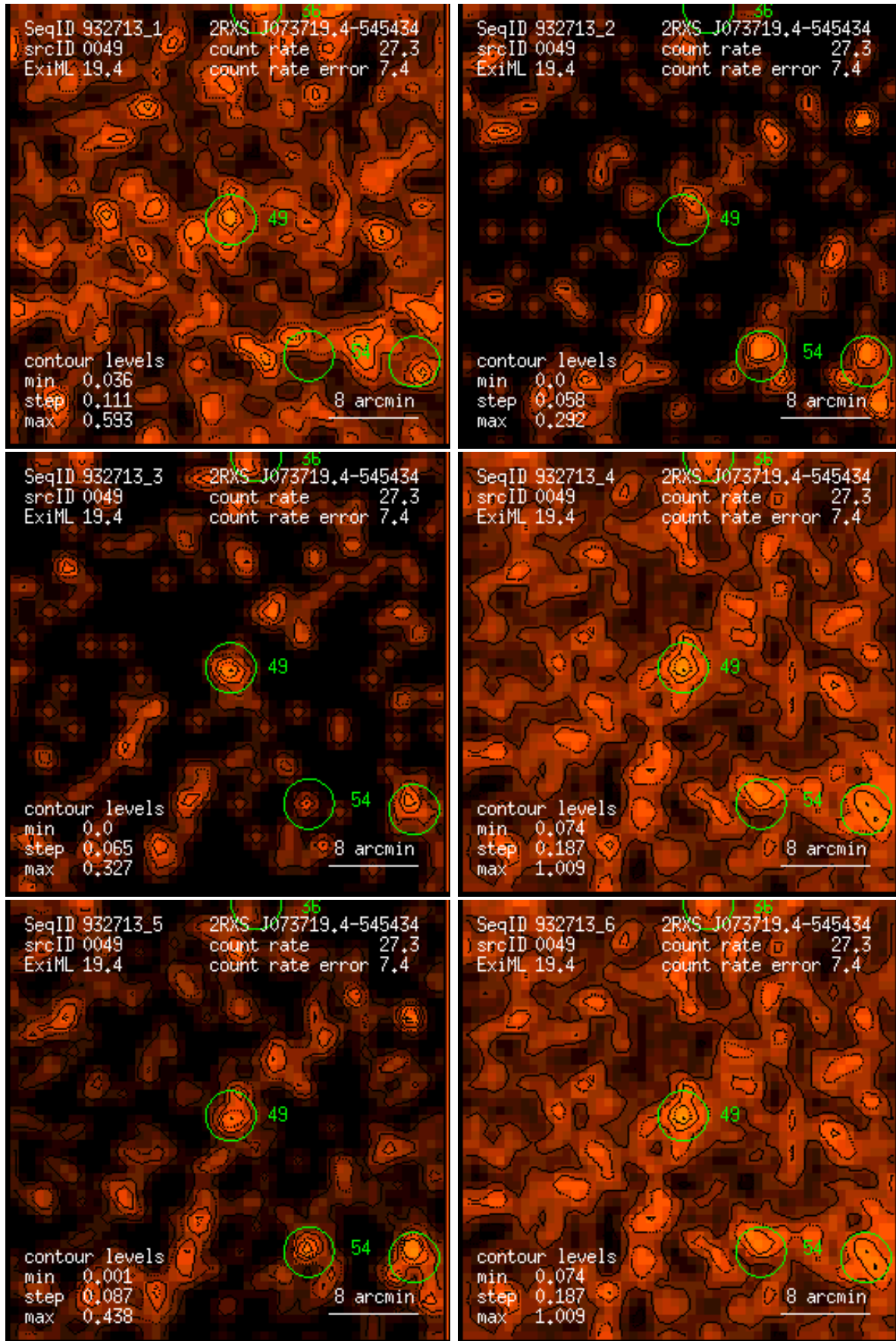
Figure 49: RASS 932713: detection 0049: band rate images, Gaussian filter: (1) PSPC channels 11 – 41, (2) 52 – 90, (3) 91 – 201, (4) 11 – 235, (5) 52 – 201, (6) 11 – 201. Broad band rates in counts/ks. Band rate contour levels in counts/ks/arcmin 2 .
