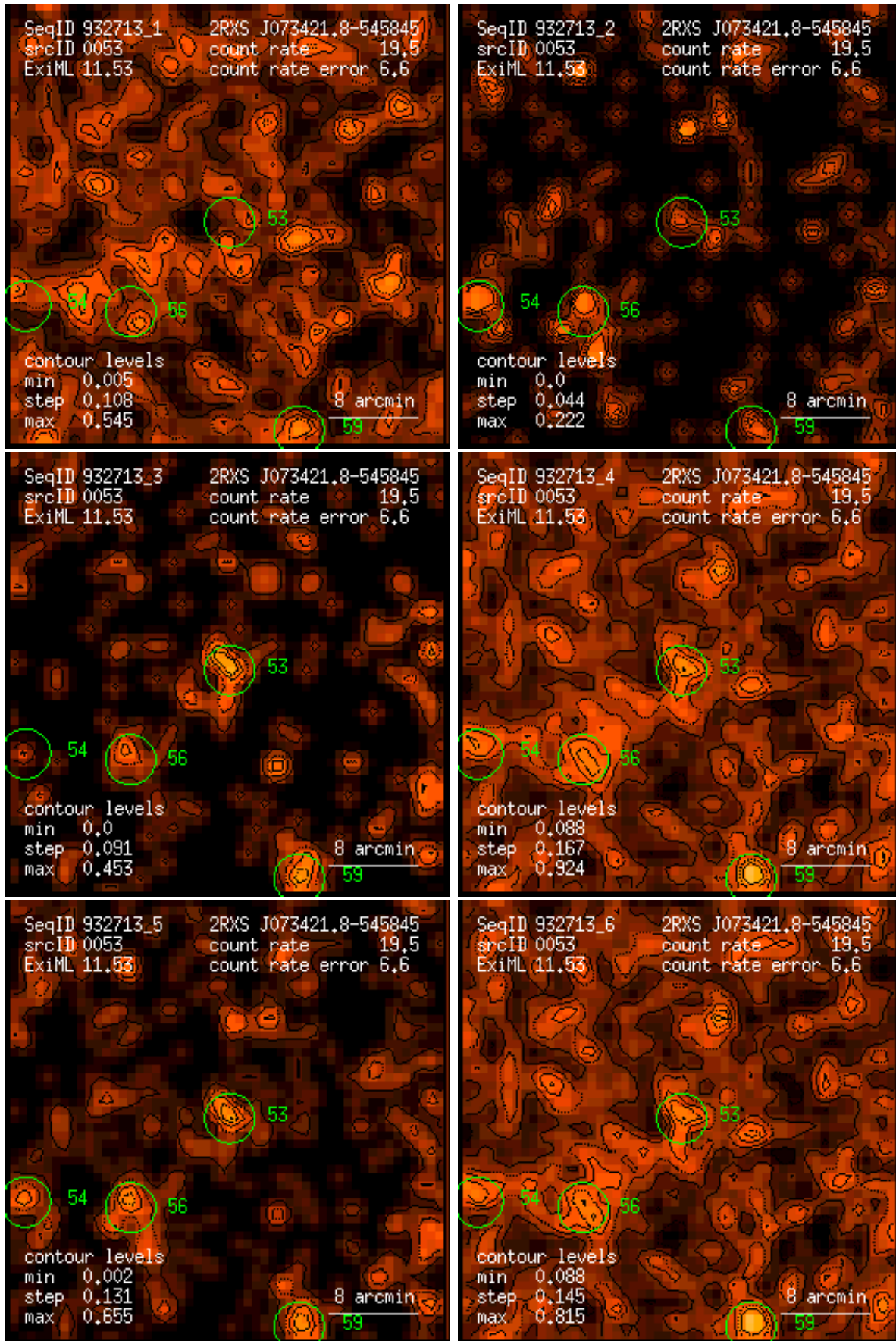
Figure 53: RASS 932713: detection 0053: band rate images, Gaussian filter: (1) PSPC channels 11 – 41, (2) 52 – 90, (3) 91 – 201, (4) 11 – 235, (5) 52 – 201, (6) 11 – 201. Broad band rates in counts/ks. Band rate contour levels in counts/ks/arcmin 2 .
