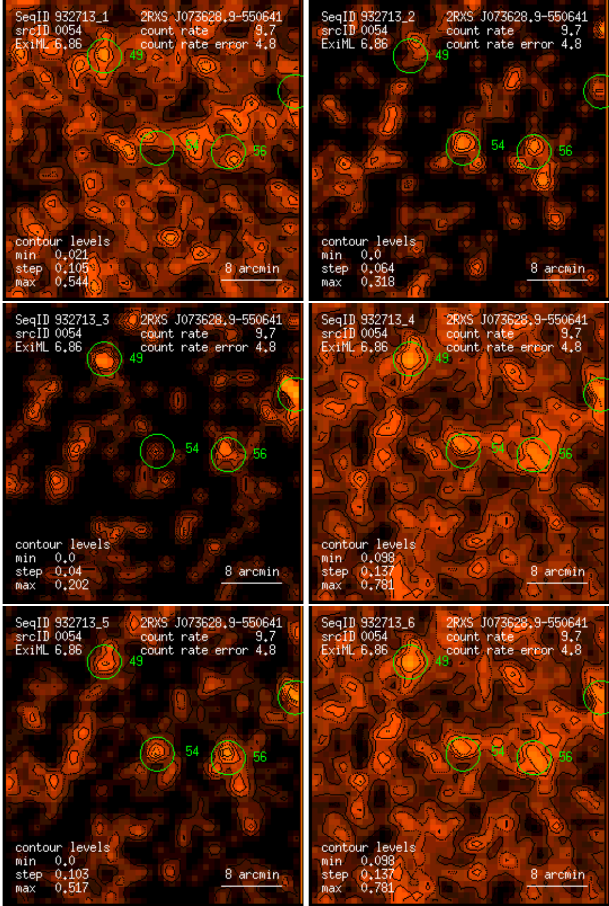
Figure 54: RASS 932713: detection 0054: band rate images, Gaussian filter: (1) PSPC channels 11 – 41, (2) 52 – 90, (3) 91 – 201, (4) 11 – 235, (5) 52 – 201, (6) 11 – 201. Broad band rates in counts/ks. Band rate contour levels in counts/ks/arcmin 2 .
