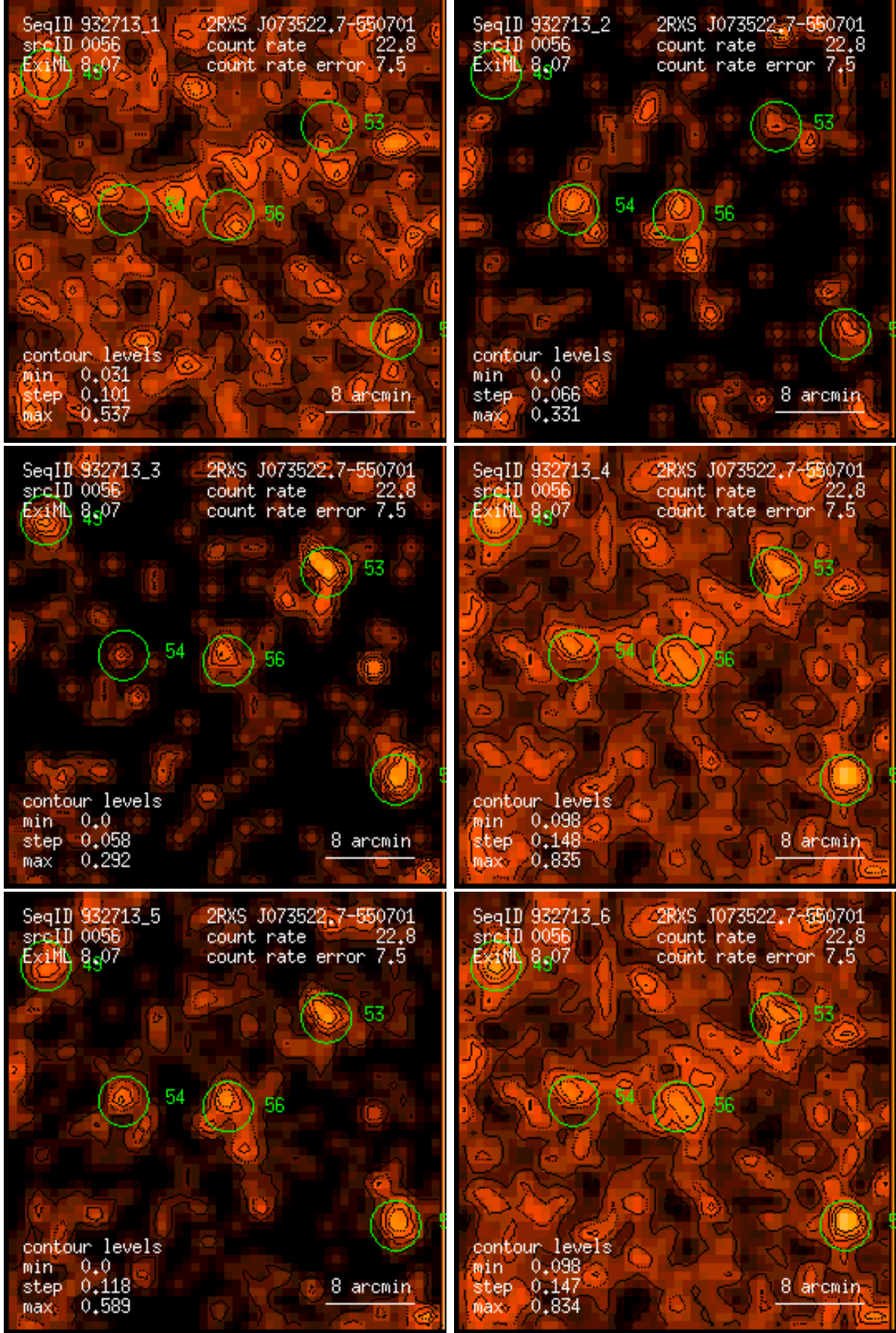
Figure 56: RASS 932713: detection 0056: band rate images, Gaussian filter: (1) PSPC channels 11 – 41, (2) 52 – 90, (3) 91 – 201, (4) 11 – 235, (5) 52 – 201, (6) 11 – 201. Broad band rates in counts/ks. Band rate contour levels in counts/ks/arcmin 2 .
