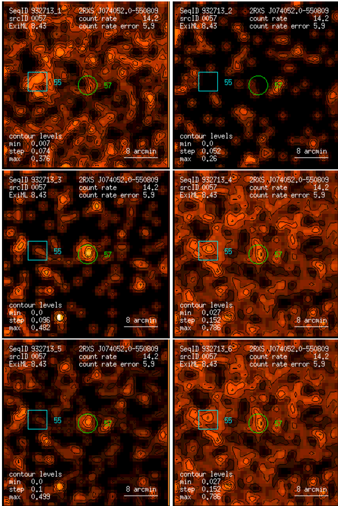
Figure 57: RASS 932713: detection 0057: band rate images, Gaussian filter: (1) PSPC channels 11 – 41, (2) 52 – 90, (3) 91 – 201, (4) 11 – 235, (5) 52 – 201, (6) 11 – 201. Broad band rates in counts/ks. Band rate contour levels in counts/ks/arcmin 2 .
